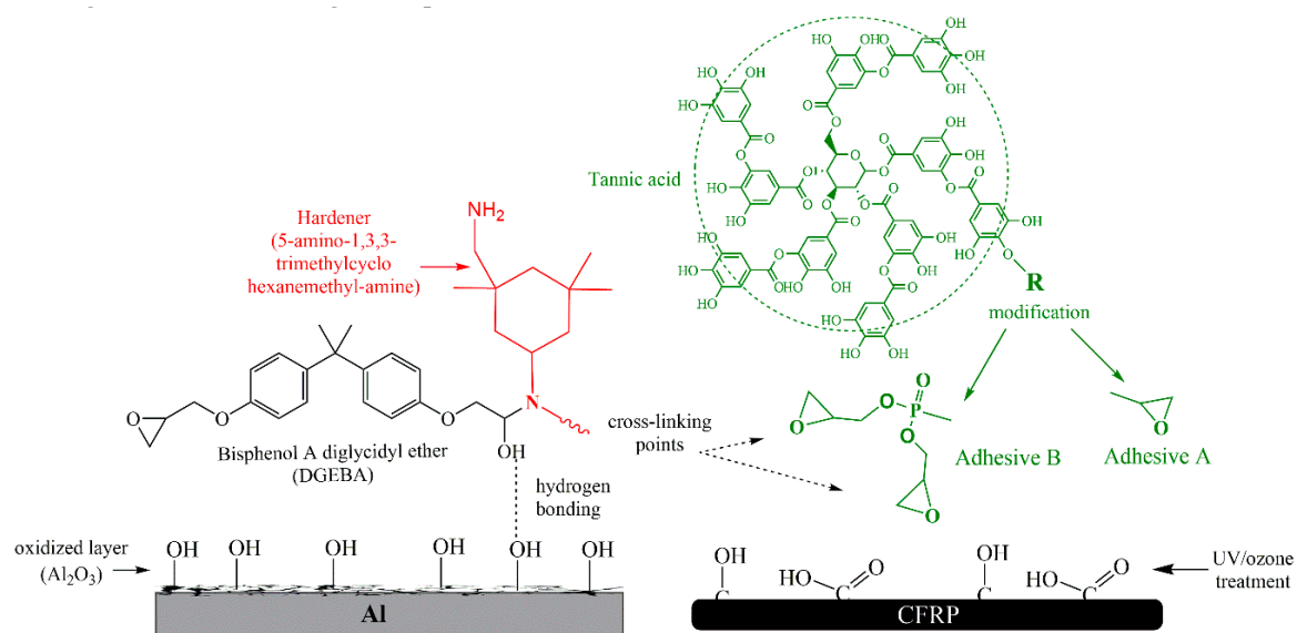
Scheme 2. Adhesive–adherend interaction for both Al and CFRP.
