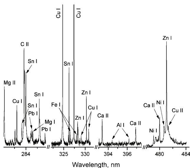
Fig. 4. LIBS spectra of bronze sample. The composition of the sample is given in Table I. The main emission lines are labeled in the spectrum. Air pressure: 0.1 mbar, laser fluence 8.6 \text{ J cm}^{-2} (intensity 30 \text{ MW cm}^{-2} ).
