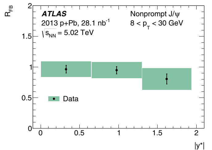
FIG. 7. (Color online) Forward-backward production ratio R_{FB} as a function of c.m. rapidity y^* for prompt J/\psi (upper panel) and nonprompt J/\psi (bottom panel). The error bars show the statistical uncertainty, and the shaded boxes show the sum in quadrature of statistical and systematic uncertainties. The two bands in the upper panel represent the predictions from Refs. [28,55] described in the text.
