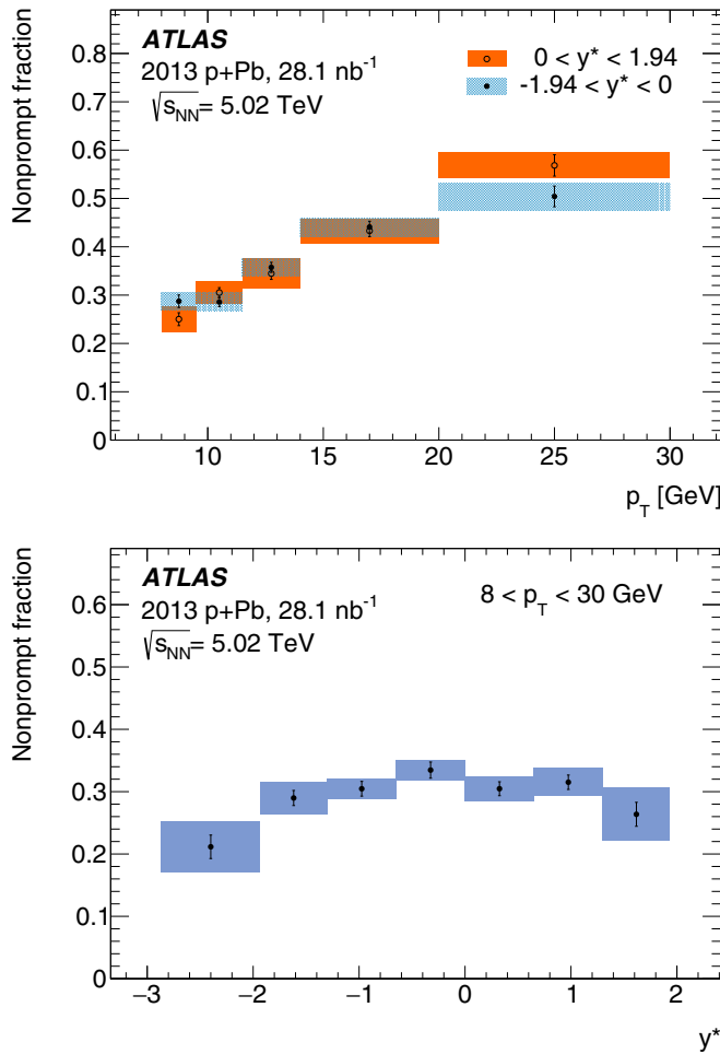
FIG. 3. (Color online) Nonprompt fraction as a function of J/\psi transverse momentum p_T (upper panel) and c.m. rapidity y^* (bottom panel). Positive y^* is defined in the proton beam direction. The error bars show the statistical uncertainty, and the shaded boxes show the sum in quadrature of statistical and systematic uncertainties.
