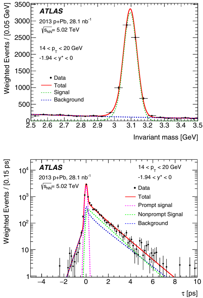
FIG. 2. (Color online) Distributions of dimuon invariant mass (upper panel) and pseudoproper time (bottom panel) of weighted J/\psi candidates in a representative interval of J/\psi transverse momentum and c.m. rapidity. The projection of the function resulting from a two-dimensional unbinned maximum-likelihood fit is also shown.
