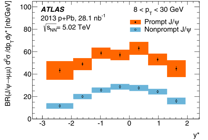
FIG. 5. (Color online) Double differential cross section for prompt and nonprompt J/\psi as a function of J/\psi c.m. rapidity y^* . Positive y^* is defined in the proton beam direction. The error bars show the statistical uncertainty, and the shaded boxes show the sum in quadrature of statistical and systematic uncertainties.
