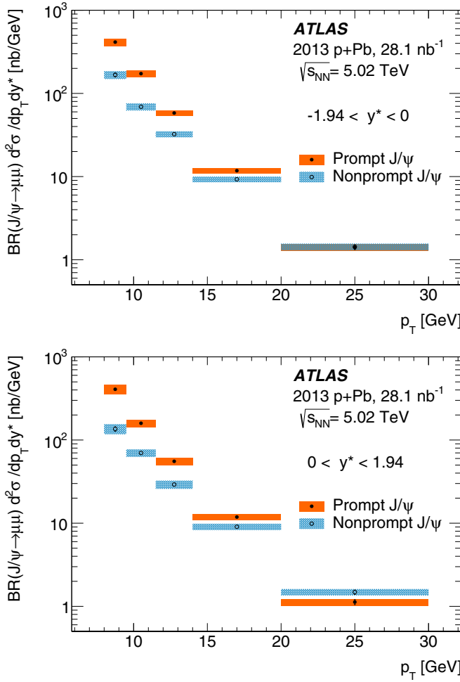
FIG. 4. (Color online) Double differential cross section for prompt and nonprompt J/\psi production as a function of J/\psi transverse momentum, p_T . The upper panel shows results in backward y^* (lead beam direction), and bottom panel in forward y^* (proton beam direction). The error bars show the statistical uncertainty, and the shaded boxes show the sum in quadrature of statistical and systematic uncertainties.
