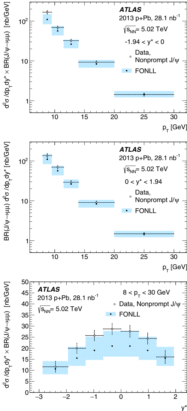
FIG. 8. (Color online) Differential cross section for production of nonprompt J/\psi as a function of J/\psi transverse momentum (upper and middle panels) and c.m. rapidity (bottom panel) compared with a FONLL calculation for pp collisions scaled by the number of nucleons in the Pb ion. Error bars represent the combination of statistical and systematic uncertainties added in quadrature. The shaded boxes represent the theoretical uncertainties on the FONLL predictions, computed as described in the text. These are strongly correlated between the bins.
