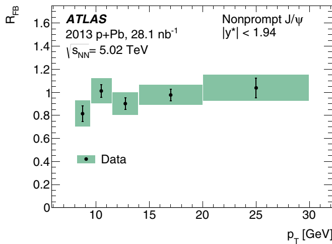
FIG. 6. (Color online) Forward-backward production ratio R_{FB} measured in the c.m. rapidity range |y^*| < 1.94 as a function of J/\psi transverse momentum for prompt J/\psi (upper panel) and nonprompt J/\psi (bottom panel). The error bars show the statistical uncertainty, and the shaded boxes show the sum in quadrature of statistical and systematic uncertainties. The narrow horizontal band in the upper panel represents the prediction from Ref. [55] described in the text.
