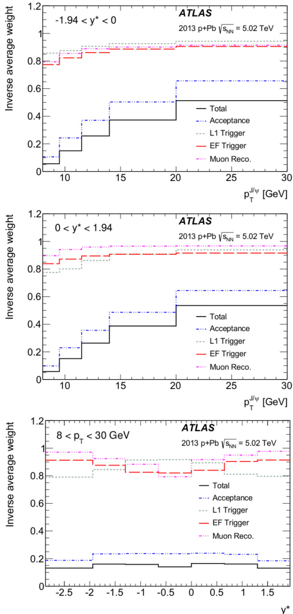
FIG. 1. (Color online) Inverse of the average weight for J/\psi candidates as a function of J/\psi transverse momentum and c.m. rapidity. The relative contributions from kinematic acceptance, reconstruction, and trigger corrections are also shown. The weights are extracted from a combination of data and MC simulation.
