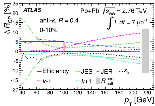
Fig. 4. Contributions to the relative systematic uncertainty on the R_{\text{CP}} from various sources for the R = 0.4 anti- k_t jets in the 0–10% centrality bin. The k \pm 1 curves denote the uncertainty due to the choice of regularization parameter obtained by unfolding with the fourth and sixth singular values. A constant 5% systematic uncertainty on the jet reconstruction efficiency is assigned for p_T < 100 GeV only. The 11% uncertainty in the determination of R_{\text{coll}} is indicated with a shaded box and is p_T -independent.
