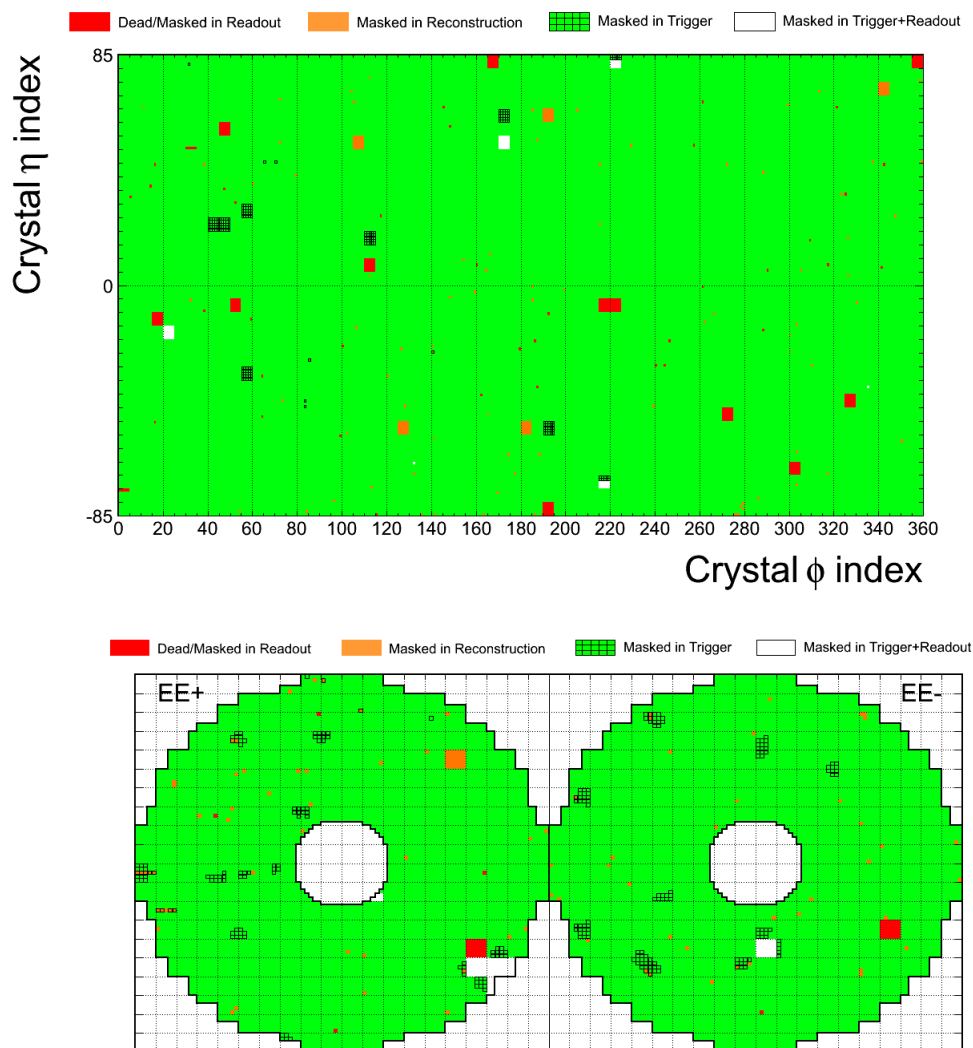
Figure 3. Distribution of masked ECAL channels in (top) barrel: \eta - \phi view of 170 \times 360 individual crystals, and (bottom) endcaps: x - y view of 2 \times 7400 individual crystals.
