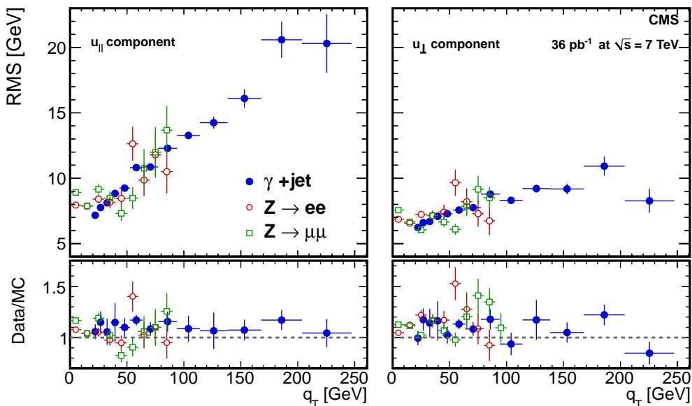
Figure 12. Resolution curves for components of hadronic recoil calculated using PF \cancel{E}_T , measured in events with one primary vertex, (left) parallel to the boson direction, and (right) perpendicular to the boson direction. Z \rightarrow \mu^+\mu^- , Z \rightarrow e^+e^- and \gamma events are indicated by open green squares, open red circles, and full blue circles, respectively. The lower frame indicates the ratio of data to simulation. The vertical axis labels at the far left apply to both subfigures.
