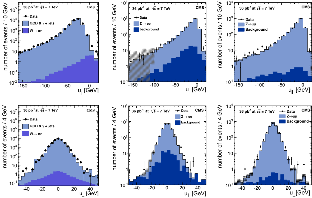
Figure 9. u_{\parallel} distributions for PF \cancel{E}_T for (top, left) \gamma , (top, middle) Z \rightarrow e^+e^- and (top, right) Z \rightarrow \mu^+\mu^- events; u_{\perp} distributions for PF \cancel{E}_T for (bottom, left) \gamma , (bottom, middle) Z \rightarrow e^+e^- , and (bottom, right) Z \rightarrow \mu^+\mu^- events. Distributions are for events containing one PV, with a correction for residual pile-up contamination. Statistical uncertainties and systematic uncertainties on the removal of events with more than one PV and on the boson q_T spectrum are shown as grey bands on the prediction from simulation. QCD refers to multijet production.
