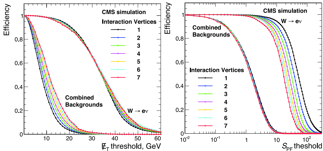
Figure 24. Efficiency versus minimum threshold curves for W \rightarrow e \nu signal and for total background for different numbers of interaction vertices with a minimum applied \cancel{E}_T threshold (left) and a minimum applied S_{PF} threshold (right).
