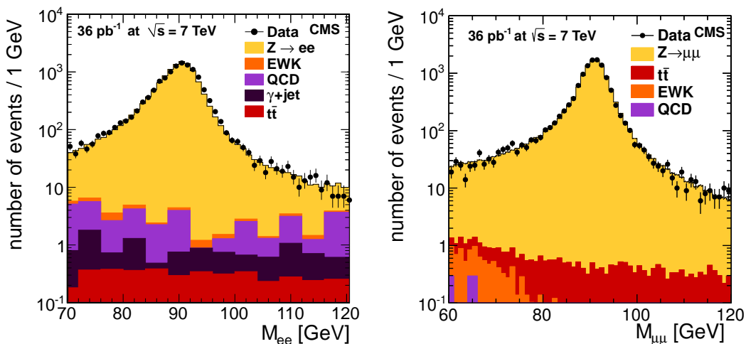
Figure 7. (left) Invariant mass distribution of the two leading electrons and (right) invariant mass distribution of the two leading muons, for the Z boson candidates, along with the predicted distributions from simulation. QCD refers to multijet events.
