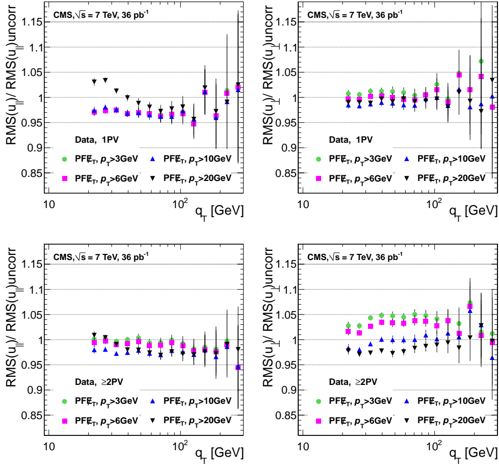
Figure 27. Ratio of PF \cancel{E}_T resolution with type-I corrections to the the PF \cancel{E}_T resolution without type-I corrections for parallel (left) and perpendicular (right) components of PF \cancel{E}_T versus \gamma q_T , for various jet correction thresholds for \gamma candidate events with 1 primary vertex (top) and more than 1 vertex (bottom) after correction for scale, using scale corrections similar to those shown in figure 10.
