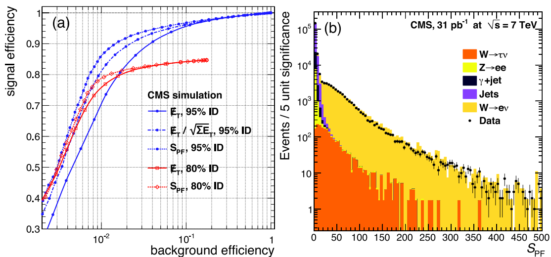
Figure 23. (left) Efficiency curves for W \rightarrow e \nu signal versus backgrounds varying the minimum value of \cancel{E}_T (solid lines), of S_{PF} (dotted lines), and of \cancel{E}_T / \sqrt{\sum E_{T_i}} (dot-dash line), with the 95% efficient (blue) or 80% efficient (red) electron isolation criterion applied. (right) Distributions of S_{PF} in candidate W \rightarrow e \nu events from data (points) and simulation (stacked histograms). The simulation components, from top to bottom, are signal (mustard) and backgrounds from jets (purple), \gamma +jets (black), Z \rightarrow e^+e^- (yellow), and W^\pm \rightarrow \tau^\pm \nu_\tau (orange). The simulation is scaled by a fit to the data with floating normalizations for the signal and the total background.
