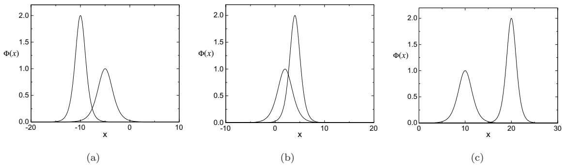
Fig. 5. The function (2.3) for \alpha = 3 . The velocities are: u = 2 (faster soliton) and u = 1 . (a) t = -5 . (b) t = 2 . (c) t = 10 .
