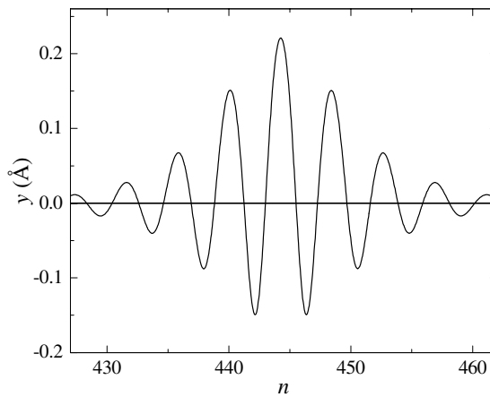
Fig. 8. The nucleotide pair stretching at t = 80 ps for: a = 1.2\text{\AA}^{\circ-1} , D = 0.07 eV, k = 12 N/m, K = 0.08 N/m, N = 10 and \eta = 0.47 .
