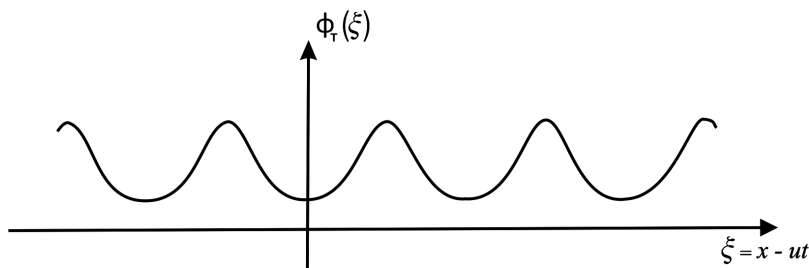
Fig. 3. A travelling wave.
