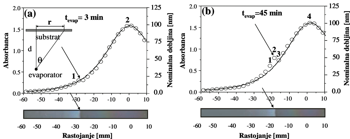
Slika 1. Apsorbancija i nominalna debljina deponovanih TPD filмова u funkciji rastojanja od nulte tačke, evaporisanih 3 (a) i 45 min (b). Brojevi predstavljaju pozicije na različitim udaljenostima od nulte tačke na kojima su izvršena merenja apsorpcionih i PL spektara i AFM snimanja; za (a): 1 – 31,0 mm, 2 – 1,0 mm; za (b): 1 – 21,0 mm, 2 – 20,0 mm, 3 – 18,0 mm, 4 – 1,0 mm. Figure 1. Absorbance and nominal thickness of deposited TPD films as functions of different distances from the zero point, evaporated for 3 (a) and (b) 45 min. Numbers represent places (distances from the zero point) at which absorption, PL spectra and AFM measurements were made; a) 1 – 31.0 mm, 2 – 1.0 mm; b) 1 – 21.0 mm, 2 – 20.0 mm, 3 – 18.0 mm, 4 – 1.0 mm.
