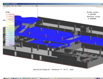
Figure 9. The 4000 ppm smoke isosurfaces after 300 seconds simulated for the “ventilated” case
