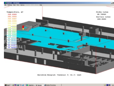
Figure 7. The 100 °C isosurfaces after 300 seconds simulated for the “ventilated” case
