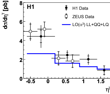
Fig. 9. Differential cross sections d\sigma/d\eta^\gamma for the inclusive isolated photon production in comparison to the previous measurement by ZEUS [17] for Q^2 > 35 \text{ GeV}^2 , E'_e > 10 \text{ GeV} , 139.8 < \theta_e < 171.9^\circ and 5 < E_T^\gamma < 10 \text{ GeV} . The additional condition W_X > 50 \text{ GeV} is used in the H1 analysis only (see Sect. 8). The cross sections are compared to the leading order, \mathcal{O}(\alpha^3 \alpha_s^0) , calculation. In contrast to the comparison in [18], the calculation is here corrected for hadronisation effects
