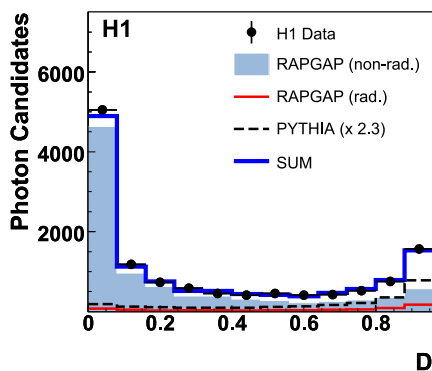
Fig. 5. The distribution of the discriminator ( D ) used in the identification of isolated photon candidates for events that have passed the event selection. The data are compared to the MC predictions described in the caption of Fig. 2
