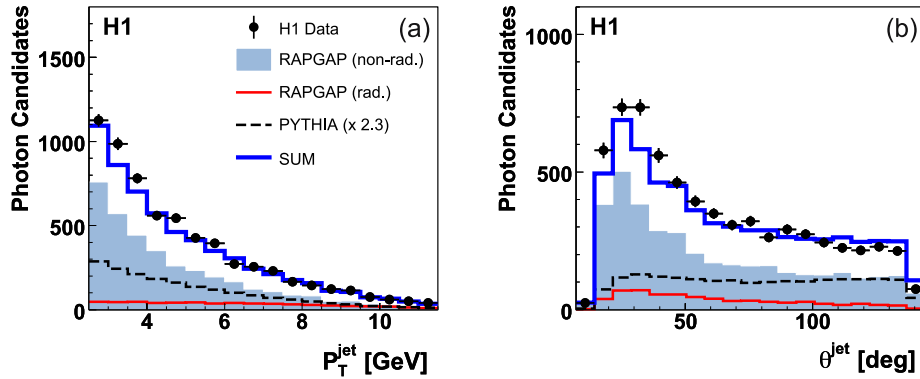
Fig. 3. Distributions of a the transverse momentum and b the polar angle of the hadronic jet with the highest transverse momentum in events with an isolated photon candidate. The data are compared to the MC predictions, as described in the caption of Fig. 2
