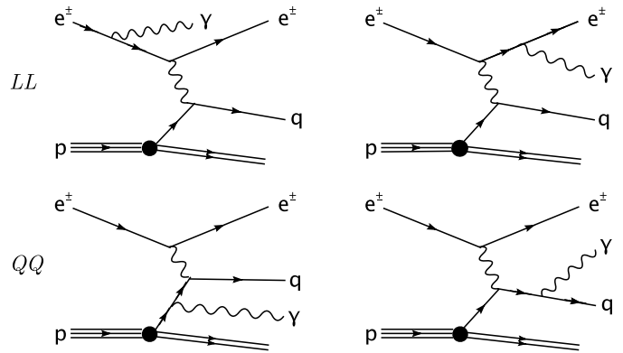
Fig. 1. Leading order diagrams for isolated photon production in DIS. The upper diagrams illustrate isolated photon production by radiation from the electron line ( LL ), while the lower diagrams correspond to production via radiation from the quark ( QQ , without the contribution from quark fragmentation)
