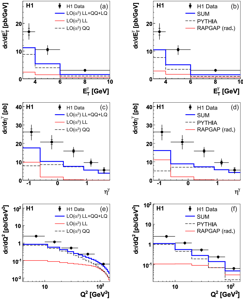
Fig. 6. Differential cross sections for inclusive isolated photon production d\sigma/dE_T^\gamma , d\sigma/d\eta^\gamma , and d\sigma/dQ^2 in the kinematic range specified in Table 1. The inner error bars on the data points indicate the statistical error, the full error bars contain in addition the systematical errors added in quadrature. The cross sections in a, c, e are shown together with a leading order, \mathcal{O}(\alpha^3\alpha_s^0) , calculation corrected for hadronisation effects, LL corresponding to radiation from the electron, QQ to radiation from the quark and LQ to their interference. The same cross sections are shown in b, d, f together with the prediction from PYTHIA for photon emission from the quark and from RAPGAP (rad.) for emission from the electron
