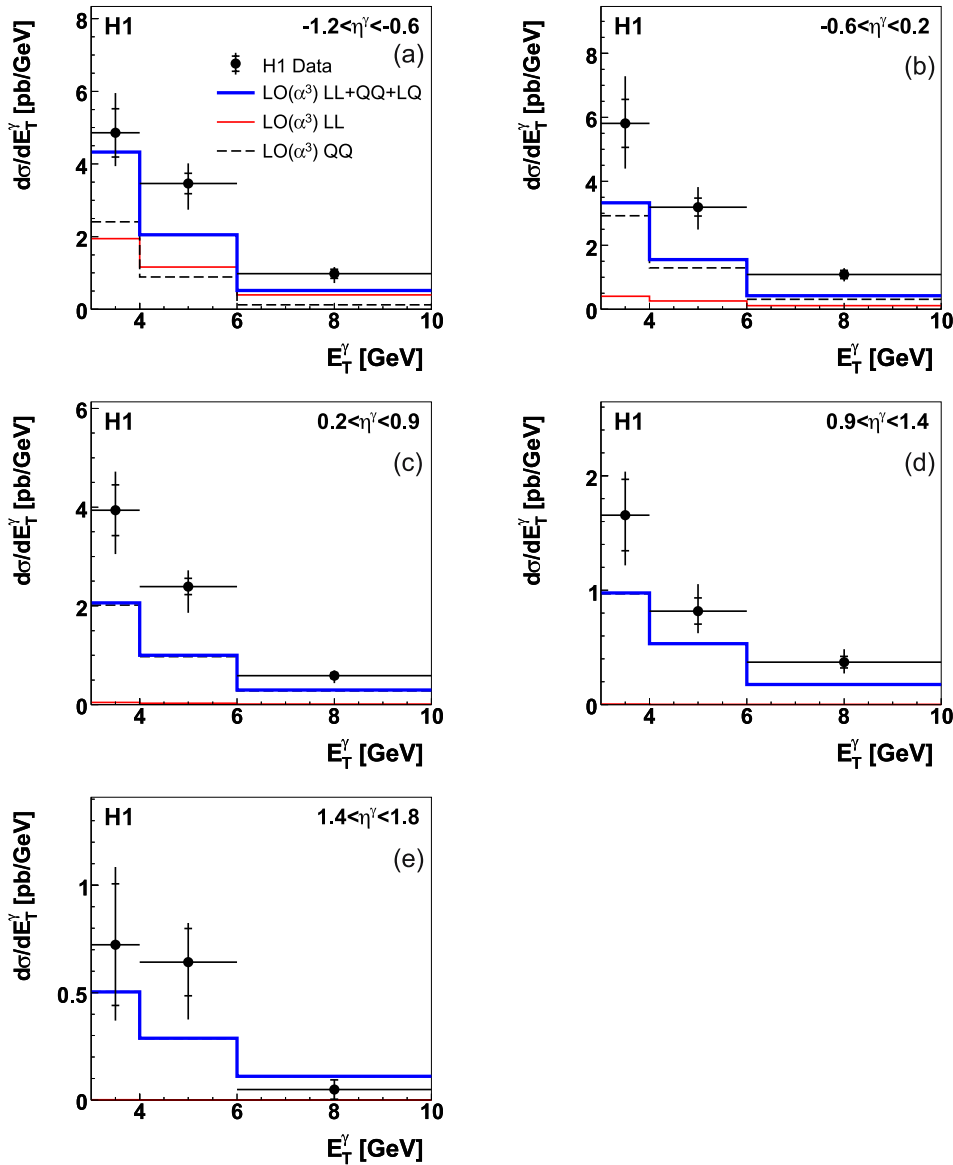
Fig. 7. Differential cross sections d\sigma/dE_T^\gamma for inclusive isolated photon production in the kinematic range specified in Table 1, in \eta^\gamma bins corresponding to the wheel structure of the LAr calorimeter (see text). The measurements are compared to a leading order \mathcal{O}(\alpha^3\alpha_s^0) calculation (more details in the caption of Fig. 6). The LL contribution is negligible for \eta^\gamma > 0.2
