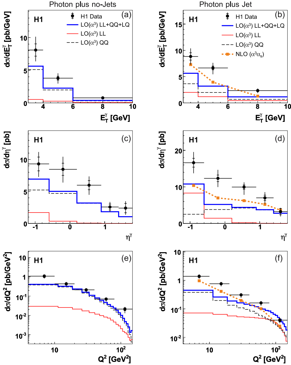
Fig. 10. Differential cross sections d\sigma/dE_T^\gamma , d\sigma/d\eta^\gamma and d\sigma/dQ^2 for photon plus no-jets (a, c, e), and photon plus jet (b, d, f) production in the kinematic range specified in Table 1. The cross sections are compared to the leading order, \mathcal{O}(\alpha^3\alpha_s^0) , calculation (more details in the caption of Fig. 6). The photon plus jet sample is additionally compared to a NLO ( \alpha^3\alpha_s ) calculation. The bin averaged NLO cross sections are indicated by the squares
