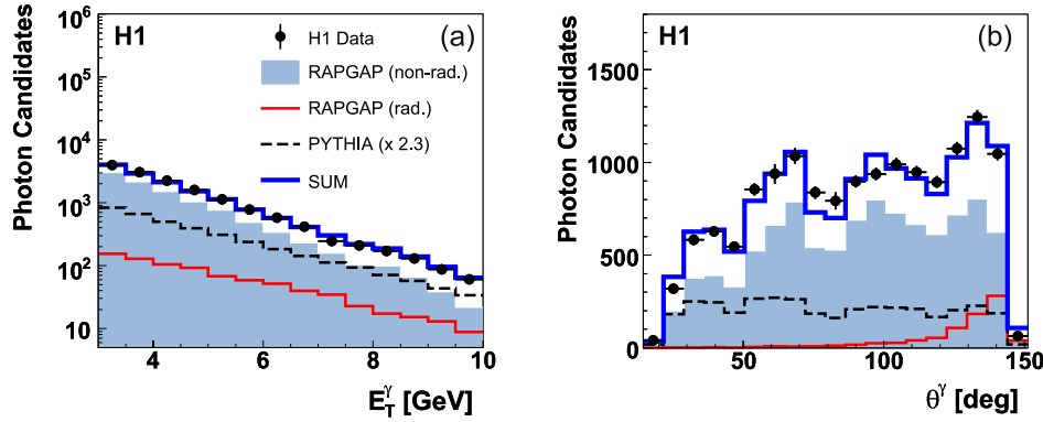
Fig. 2. Distributions of a E_T^\gamma and b \theta^\gamma for isolated photon candidates in the final event sample. Data are shown as points with error bars . The bold solid histogram shows the sum of the expectation from RAPGAP (non-rad.) for neutral hadron background ( shaded ), from PYTHIA for radiation from the quark scaled by a factor of 2.3 ( dashed line ) and from RAPGAP (rad.) for radiation from the electron ( solid line ). The unshaded area corresponds to the estimated isolated photon contribution (RAPGAP(rad.) plus PYTHIA \times 2.3 )
