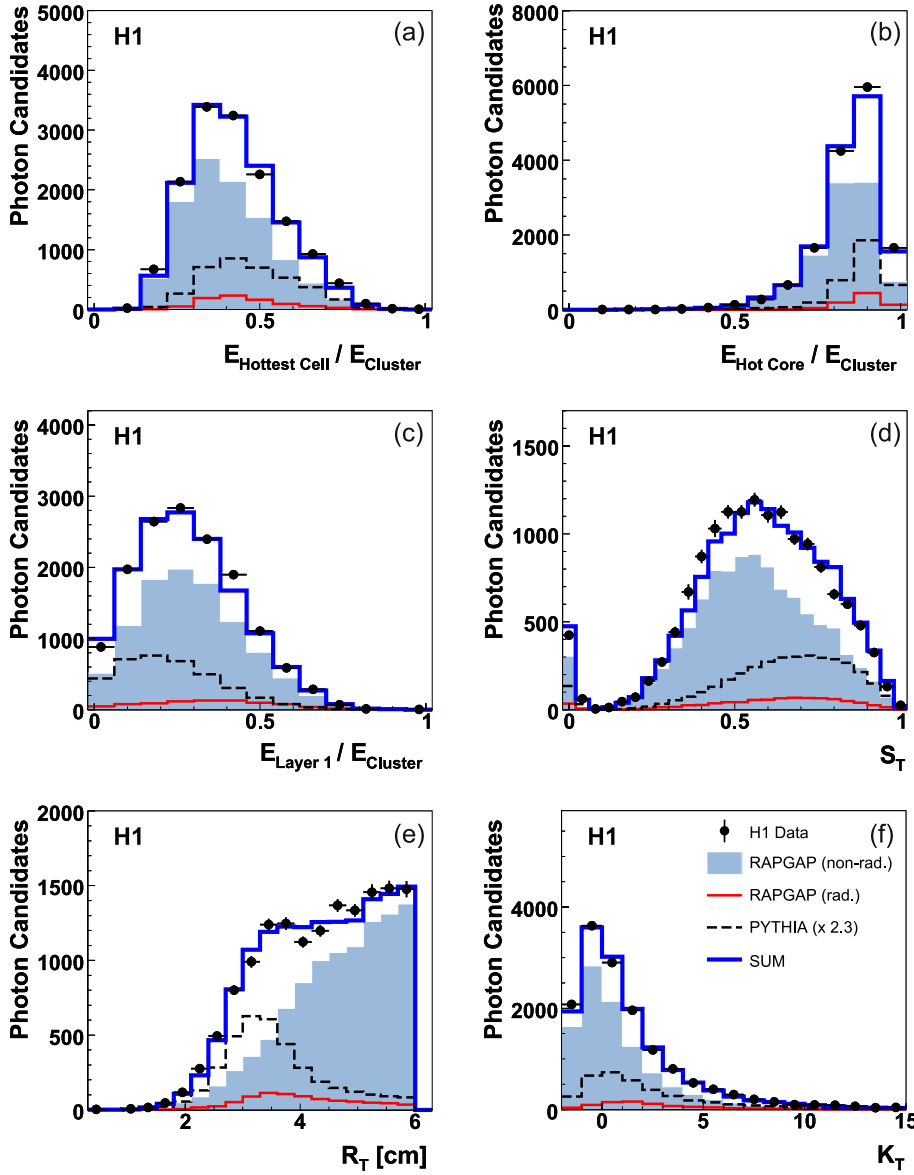
Fig. 4. Distributions of the six variables that are used to define the discriminant for isolated photon identification: a hottest cell fraction, b fraction of the hot core, c first layer fraction, d transverse symmetry S_T , e transverse radius R_T and f transverse kurtosis K_T . The data are shown with the MC predictions described in the caption to Fig. 2. The shape difference between RAPGAP (rad.) and PYTHIA arises from the different distributions in phase space (see Fig. 2b)
