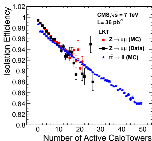
Figure 32. Muon isolation efficiency versus number of calorimeter towers in the region of |\eta| < 2.7 having transverse energy larger than 1 GeV. Results for muons with 20 < p_T < 50 GeV/c from Z decays obtained in data and in simulation are compared with the efficiency for prompt muons in a simulated sample of top pairs decaying leptonically. All results were obtained with the LKT method using the I_{\text{comb}}^{\text{rel}} algorithm with a threshold of 0.15. The MC samples include simulation of pile-up events.
