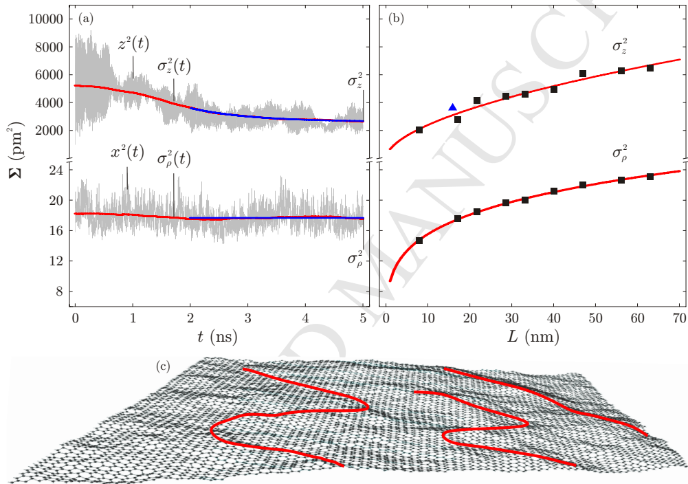
Figure 2: (a) Dependencies of the atom mean squared displacements (the gray lines), and covariance matrix components (the red lines) on time for graphene at T = 300 K. The blue lines show fits of covariance matrix components only for the atom steady state motion. (b) Solid black squares show scaling of the equilibrium covariance matrix components with the linear supercell size L , red lines are fits by the power law AL^\zeta . Solid blue triangle shows the result of the simulation from the Ref. [22]. (c) State of the graphene sheet at t = 2.9 ns. Major ripples are denoted by thick red lines.
