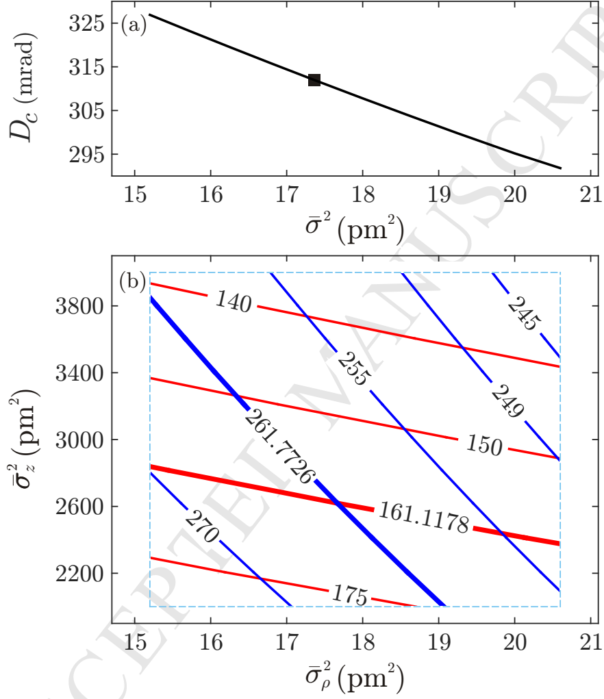
Figure 7: (color online) (a) Dependency of the rainbow diameter D_c on the variance \bar{\sigma}^2 , in the case of the normal incidence. Square marker indicate diameter of the rainbow c from the Fig. 3(a). (b) Blue lines represent level lines of the rainbow diameter D_c(\bar{\sigma}_\rho, \bar{\sigma}_z) in the case of normal incidence. Red lines represent level lines of rainbow minor diameter D_e^m(\bar{\sigma}_\rho, \bar{\sigma}_z) for the sample tilted by the angle \Theta = 0.065\pi rad. Boundaries of the domain are shown by dashed blue lines. Level values are expressed in mrad. Thick blue and red lines show corresponding diameters of the rainbows c and e from the Figs. 5(a) and (b) respectively.
