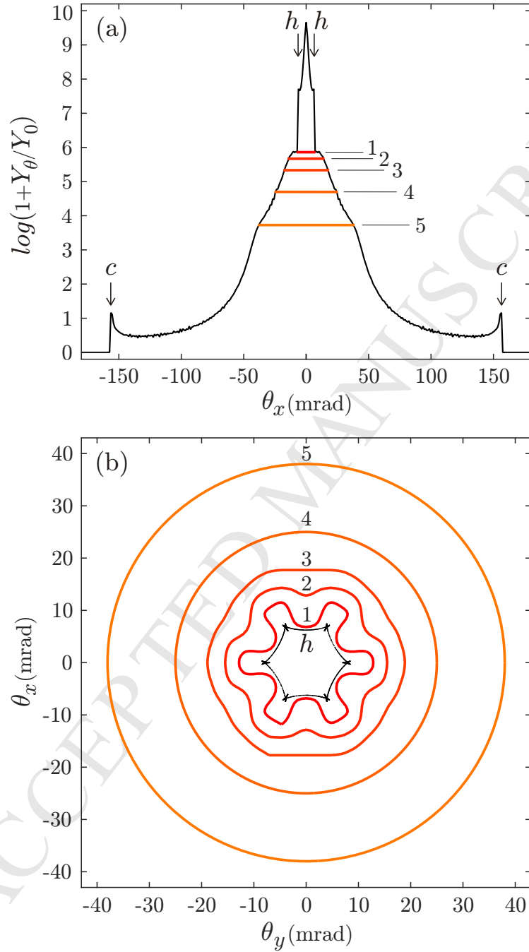
Figure 4: (a) The vertical slice through angular distribution from Fig. 3(a) where normalization factor Y_0 is 1/\text{mrad}^2 . (b) Filtered iso-level lines of the distribution from Fig. 3(a) in the vicinity of the rainbow line h .
