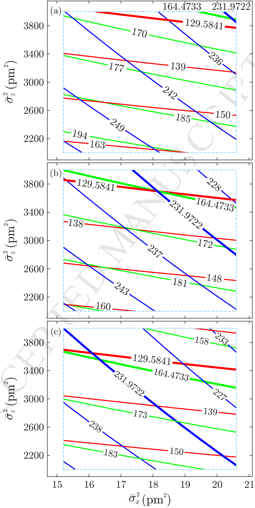
Figure 8: (color online) The blue, red and green lines represent cross-sections through level surfaces of the rainbow diameter D_e^M(\bar{\sigma}_x, \bar{\sigma}_y, \bar{\sigma}_z) in the case of normal incidence \mathcal{D}_e^M(\bar{\sigma}_x, \bar{\sigma}_y, \bar{\sigma}_z) in the case of sample tilted by the angle \Theta = 0.065\pi , and \mathcal{D}_e^M(\bar{\sigma}_x, \bar{\sigma}_y, \bar{\sigma}_z) in the case sample additionally rotated by the angle \Phi = 0.25\pi , respectively, for: (a) \bar{\sigma}_x = 30.00 \text{ pm}^2 , (b) \bar{\sigma}_x = 35.45 \text{ pm}^2 , and (c) \bar{\sigma}_x = 40.00 \text{ pm}^2 . Boundaries of the domain are shown by dashed blue lines. Level values are expressed in mrad. Thicker blue and red lines show corresponding diameters of the rainbows from the Figs. 6(a), (b) and (c) respectively.
