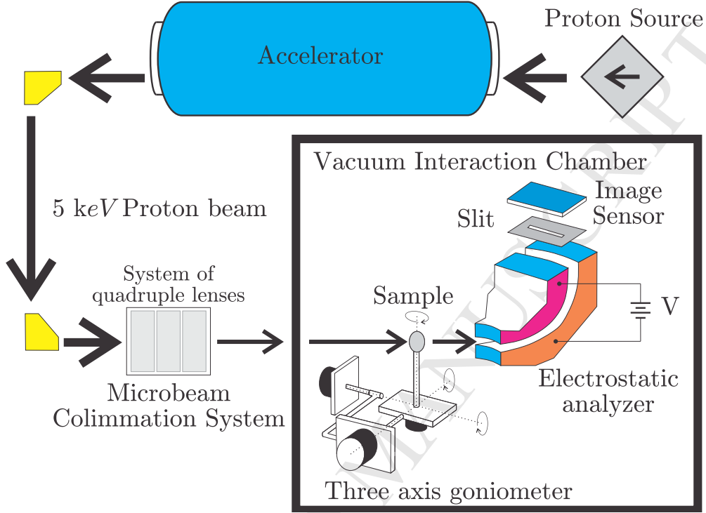
Figure 1: Schematics of the experimental setup.
