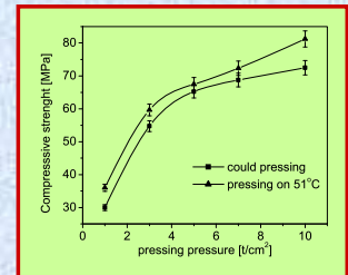
Fig 2. Compressive strength dependence on processing pressure and temperature
