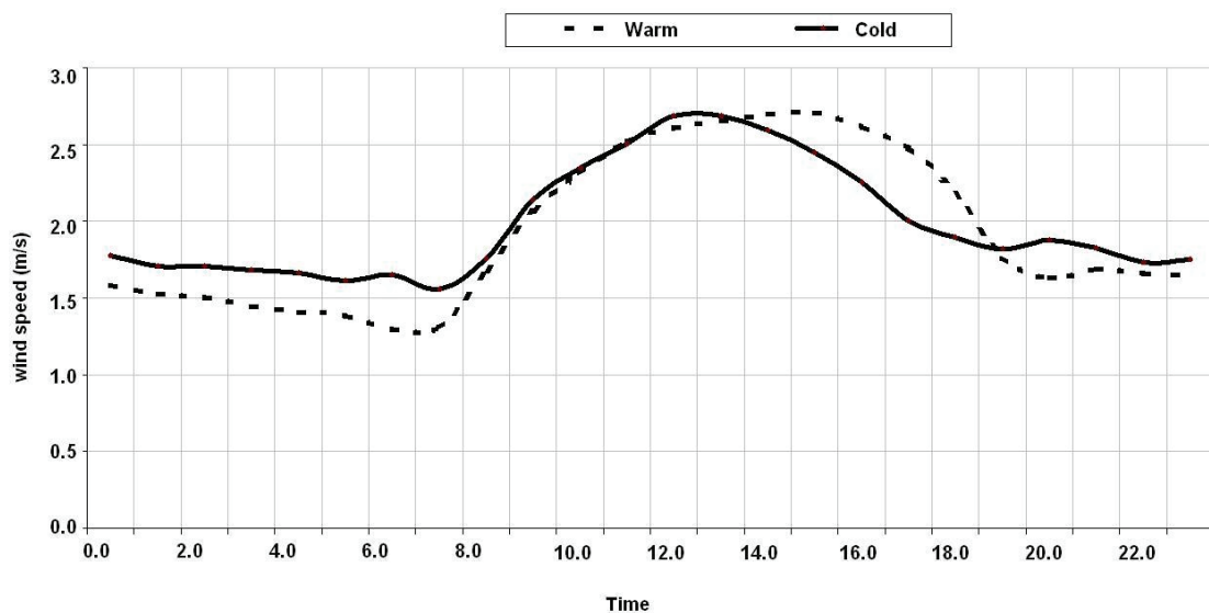
Figure 3. Diurnal time pattern of wind speed at measuring point Park in 2010.
