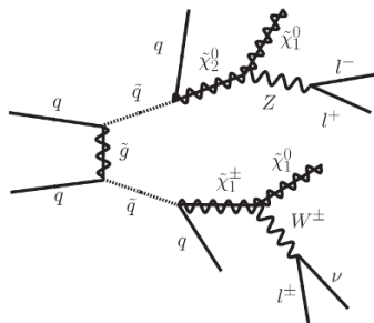
Figure 8. Feynman diagram of cascade topology denoted in supersymmetric nomenclature. The analysis is done with WW, ZZ and WZ combinations of weak vector bosons; WZ is shown in the diagram. This topology may also be found in other models such as UED.
