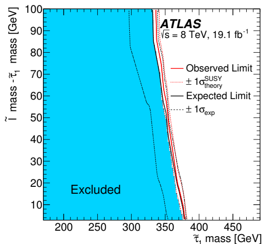
Figure 6. 95% CL excluded regions for directly produced sleptons in the plane m(\tilde{\ell}) - m(\tilde{\tau}_1) vs. m(\tilde{\tau}_1) . The excluded region is shown in blue. The expected limit is drawn as a solid black line with a \pm 1\sigma uncertainty band drawn as dashed black lines. The observed limit is shown as solid red line with a \pm 1\sigma uncertainty band drawn as dashed red lines.
