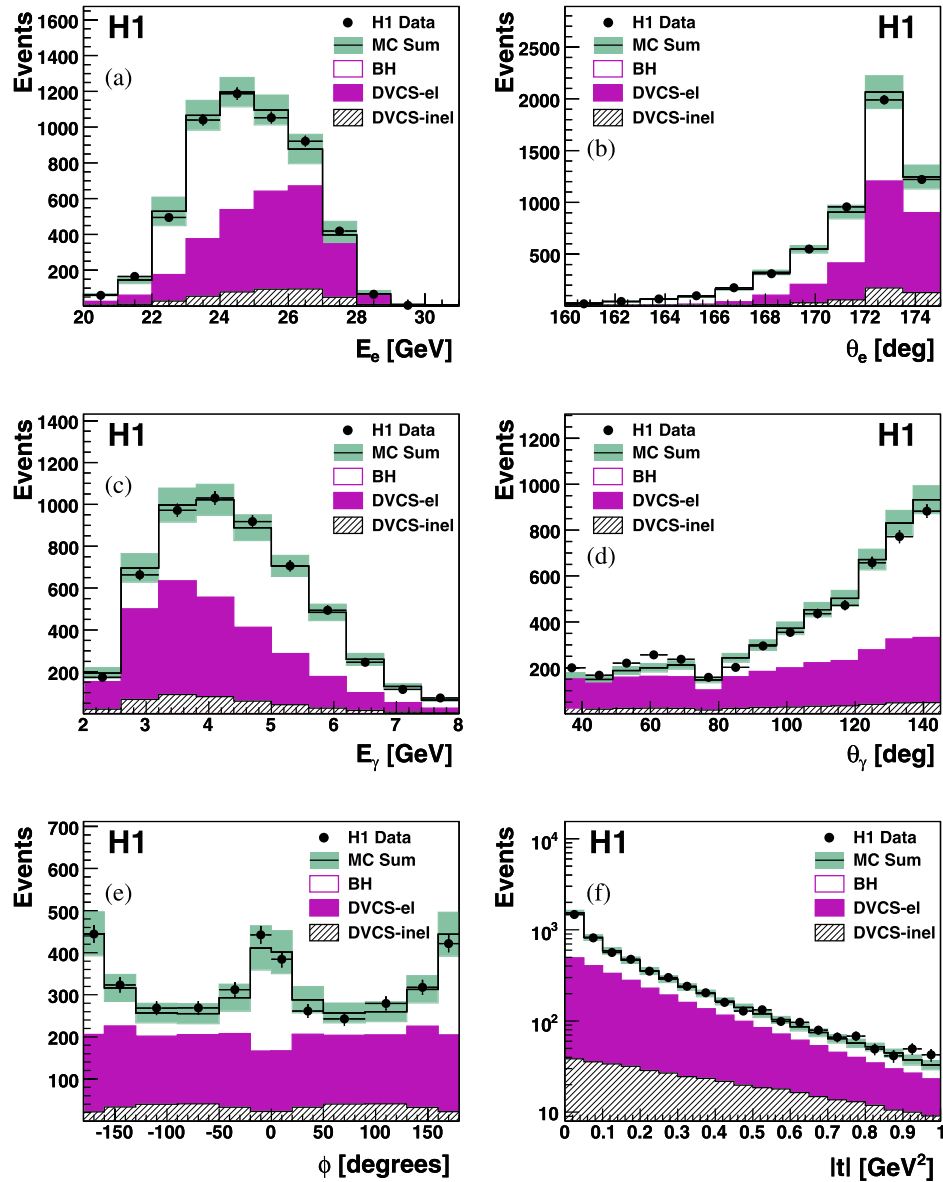
Fig. 1. Distributions of the energy (a) and polar angle (b) of the scattered electron, the energy (c) and polar angle (d) of the photon, the \phi azimuthal angle between the plane of incoming and outgoing lepton and the plane of virtual and real photon [2] (e) and the proton four momentum transfer squared |t| (f). The data correspond to the full e^\pm p sample and are compared to Monte Carlo expectations for elastic DVCS, elastic and inelastic BH and inelastic DVCS. All Monte Carlo simulations are normalised according to the luminosity of the data. The open histogram shows the total prediction and the shaded band its estimated uncertainty.
