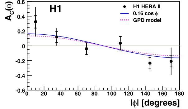
Fig. 6. Beam charge asymmetry as a function of the angle \phi as defined in [2], integrated over the kinematic range of the analysis. The inner error bars represent the statistical errors, the outer error bars the statistical and systematic errors added in quadrature. The function 0.16 \cos \phi is also shown (solid line), together with the GPD model prediction (dashed line).
