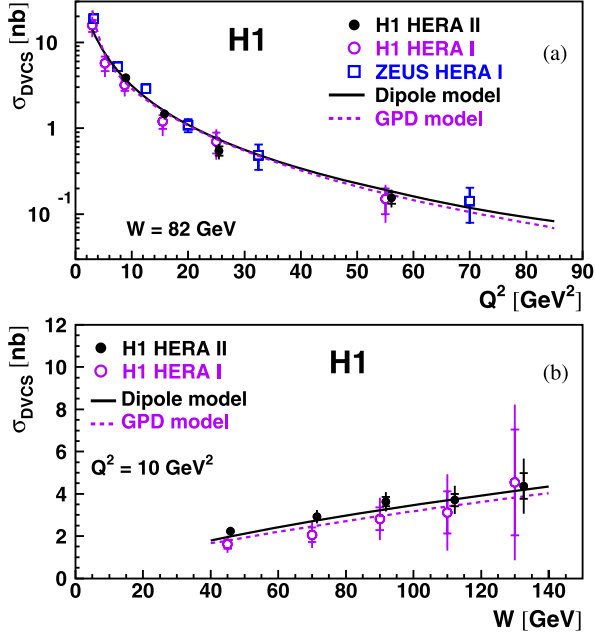
Fig. 2. The DVCS cross section \gamma^*p \rightarrow \gamma p as a function of Q^2 at W = 82 \text{ GeV} (a) and as a function of W at Q^2 = 10 \text{ GeV}^2 (b). The results from the previous H1 [10] and ZEUS [12] publications based on HERA I data are also displayed. ZEUS measurements are propagated from W = 104 \text{ GeV} to 82 \text{ GeV} using a W^{0.52} . The inner error bars represent the statistical errors, the outer error bars the statistical and systematic errors added in quadrature. The dashed line represents the prediction of the GPD model [6] and the solid line the prediction of the dipole model [15].
