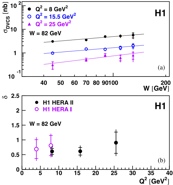
Fig. 3. The DVCS cross section \gamma^*p \rightarrow \gamma p as a function of W at three values of Q^2 (a). The solid lines represent the results of fits of the form W^\delta . The fitted values of \delta(Q^2) are shown in (b) together with the values obtained using HERA I data [10]. The inner error bars represent the statistical errors, the outer error bars the statistical and systematic errors added in quadrature.
