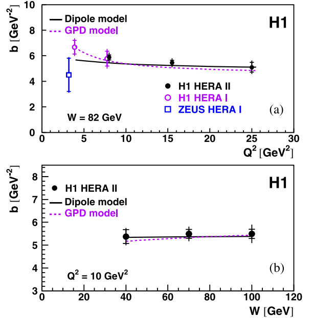
Fig. 4. The fitted t -slope parameters b(Q^2) are shown in (a) together with the t -slope parameters from the previous H1 [10] and ZEUS [12] publications based on HERA I data. In (b) the fitted t -slope parameters b(W) are shown. The inner error bars represent the statistical errors and the outer error bars the statistical and systematic errors added in quadrature. The dashed line represents the prediction of the GPD model [6] and the solid line the prediction of the dipole model [15].
