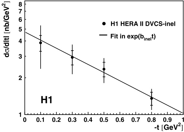
Fig. 5. The inelastic DVCS cross section differential in t at W = 82 GeV and Q^2 = 10 GeV 2 and for events with 1.4 \lesssim M_Y \lesssim 10 GeV. The inner error bars represent the statistical errors, the outer error bars the statistical and systematic errors added in quadrature.
