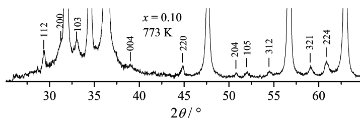
Fig. 2. X-Ray diffraction pattern at 300 K for the Zn–Mn–O sample with x = 0.10 thermally treated at 773 K recorded at a slow scan rate. The vertical ticks and indices in the spectrum indicate the peak positions of tetragonal \text{ZnMn}_2\text{O}_4 .
