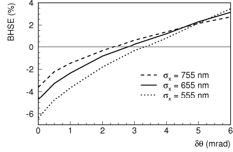
Figure 3. BHSE as a function of \delta\theta for different horizontal bunch sizes \sigma_x
