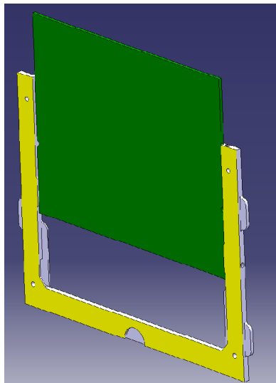
Figure 3. PermaGlass frame as holder for the existing LumiCal sensor board.
