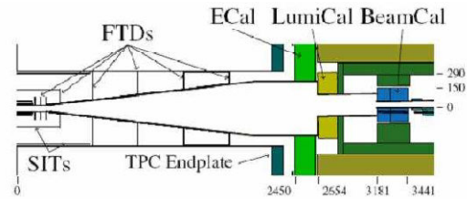
Figure 1. Forward Tracking and Calorimeters seen from the top.
