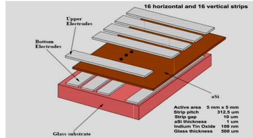
Figure 5. The DPSD-515 amorphous silicon strip sensor with 16 horizontal and vertical strips.
