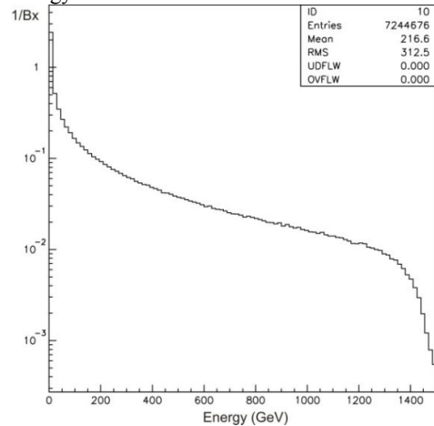
Figure 9. Energy distribution of photons generated using GuineaPig.
