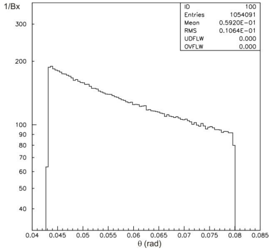
Figure 6. \theta distribution of incoherent pairs in the fiducial volume of LumiCal
