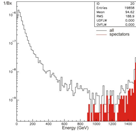
Figure 4. Energy distribution of leptons from physics background in the fiducial volume of LumiCal
