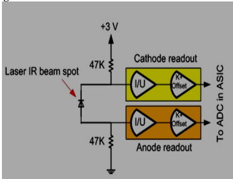
Figure 8. The scheme view of readout electronics
