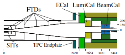
Figure 1. The very forward region of the CLIC detector
