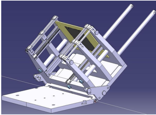
Figure 7. Proposed solution to allow the use of the mechanical infrastructure both for horizontal beams and cosmic (vertical) muons.
