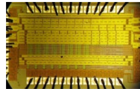
Figure 3. Photograph of glued and bonded front-end ASIC prototype.
