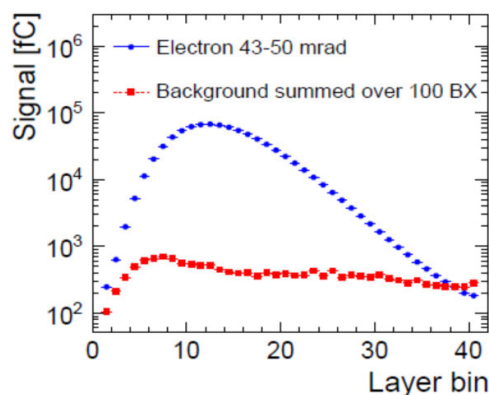
Figure 2. The energy profile of a shower of an Electron from Bhabha scattering and of background depositions as a function of the depth in LumiCal
