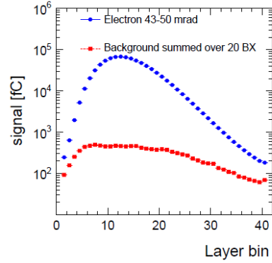
Figure 3. Charge deposit profile of the e^- signal (blue dots) as a function of the layer number in LumiCal, overlaid with background signal in e^- pads (red squares), summed over 20 BX.
