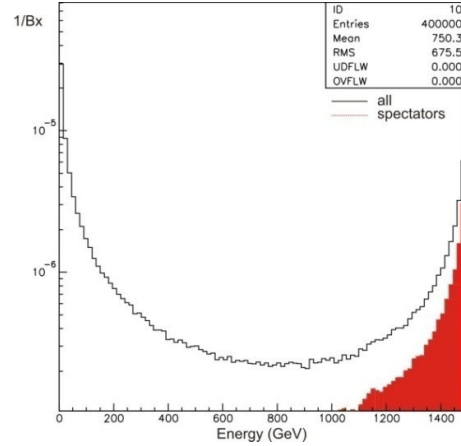
Figure 2. Energy distribution of leptons from physics background in the full angular range.
