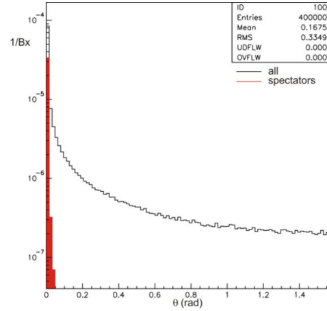
Figure 3. \theta distribution of leptons from physics background in the full angular range
