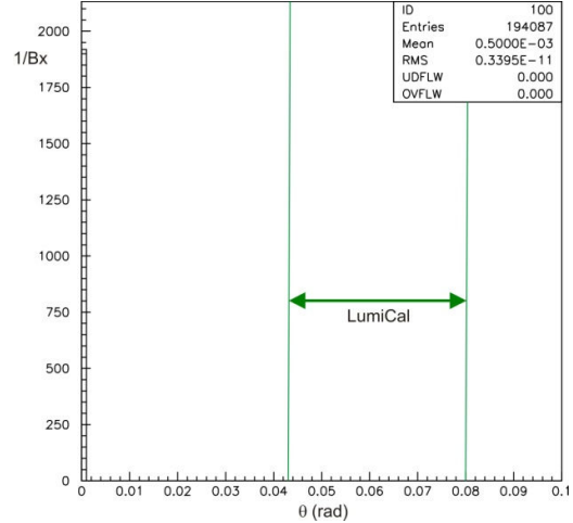
Figure 8. \theta distribution of incoherent pairs carrying the energy above 60% of the beam energy
