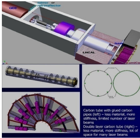
Figure 3. Top: The QD0 magnet as reference frame for LumiCal alignment. Bottom: The possible localization of the additional carbon pipes for laser beams from tunable laser. The transparent sensors can be placed on the disks of vertex detectors.
