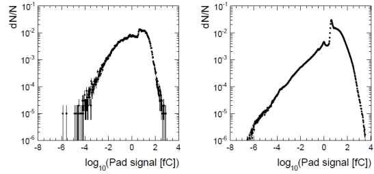
Figure 4. Left: distribution of charge depositions in a single pad from incoherent pairs. Right: same for \gamma\gamma
