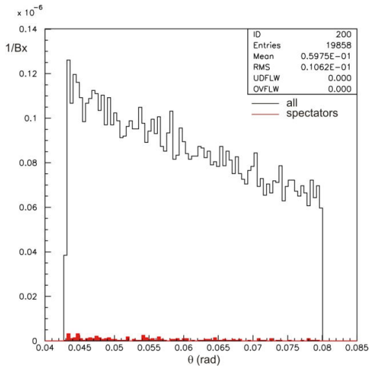
Figure 5. \theta distribution of leptons from physics background in the fiducial volume of LumiCal
