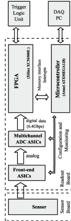
Figure 2. Readout system block diagram.
