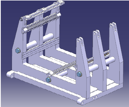
Figure 2. The modified wider version of the mechanical infrastructure, designed to accommodate the existing sensor board.
