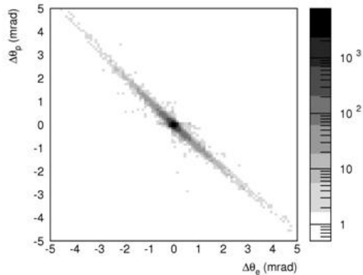
Figure 1. Correlation between the polar-angle shifts of the outgoing electron and positron in Bhabha scattering under influence of the Beamstrahlung effect
