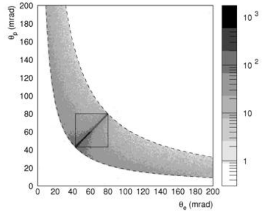
Figure 4. Histogram of the polar angles of the outgoing electron and positron from the Bhabha scattering at CLIC. The rectangular frame from 43 to 80 mrad represents the fiducial volume of the LumiCal.
