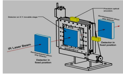
Figure 9. Proposed experimental set-up with transparent DPSD sensors for laboratory and test beam measurements
