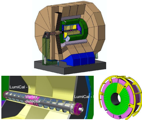
Figure 1. Top: ILD detector; Bottom: Inner subdetectors: luminosity and vertex detectors together with the support tube (in grey). In addition one of the Lumical calorimeter is shown.
