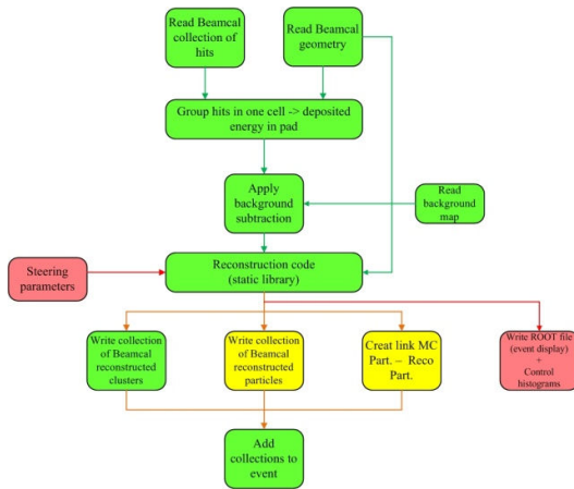
Figure 3. The electron reconstruction algorithm in the beam calorimeter is shown as a flow chart.
