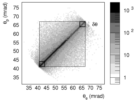
Figure 2. 2D histogram plot of the polar angles of the outgoing Bhabha positrons versus the electrons. Selection cuts to the fiducial volume were applied before including the Beamstrahlung effect. The two thick boxes represent the areas the most affected by the BHSE.
