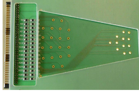
Figure 6. Sensor mounted on fan-out and instrumented by capacitances, resistors and connector.
