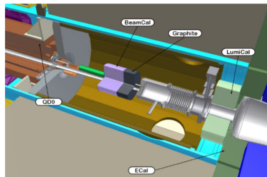
Figure 1. The very forward region of a detector at CLIC. LumiCal is positioned just behind the electromagnetic calorimeter and BeamCal in front of the beam focusing magnet.
