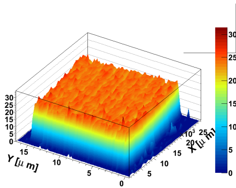
Figure 8. The average signal divided by the MPV as a function of hit position.
