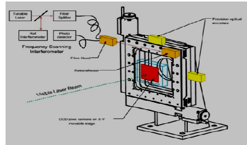
Figure 10. Proposed setup with FSI for laboratory and test beam measurements.
