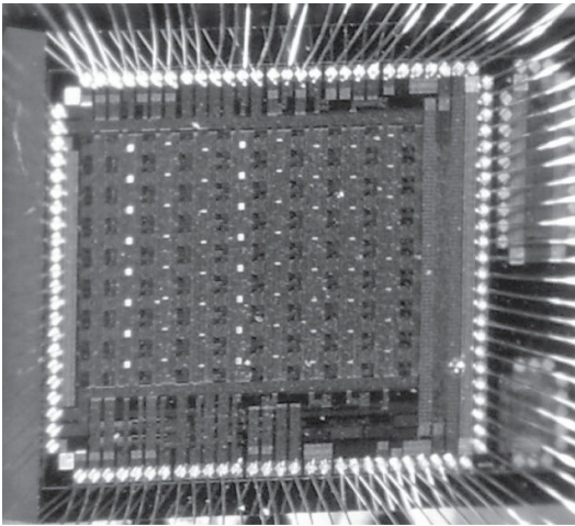
Figure 4. Micrograph of prototype ASIC bonded.
