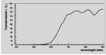
Figure 7. DPSD-516: The transmission as a function of wavelength.
