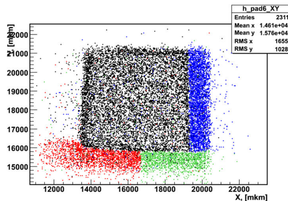
Figure 3. The distribution of hits on a fully instrumented sensor of BeamCal.
