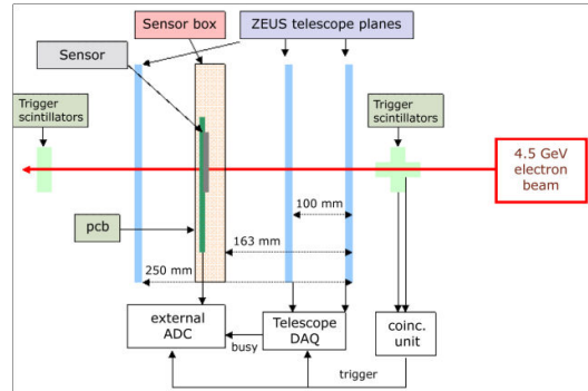
Figure 1. Test beam setup and connection scheme.
