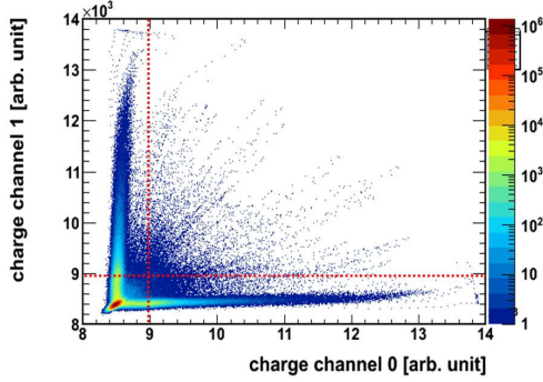
Figure 5. Point-by-point 2D correlation plot. The significant area of cross-talk is estimated between the outer x-y axes (black) and inner axes (red).
