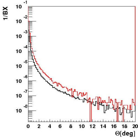
Figure 1. Polar angle distributions of final state particles with E > 0.6E_{\text{beam}} from four-fermion processes, at the center-of-mass energy of 500 GeV (red) and 1 TeV (black).
