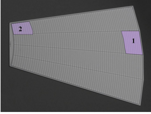
Figure 2. Tail of the silicon sensor prototype. Measured areas (1 and 2) are highlighted.
