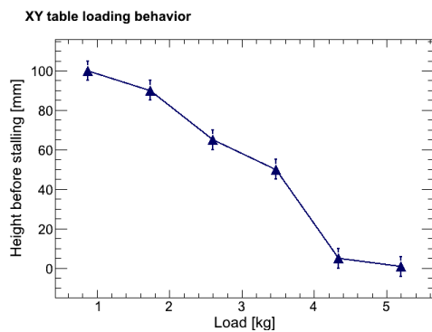
Figure 3. As the weight of the load increases (x-axis), the maximum height able to be reached by the table goes down to almost zero at 5 kg.
