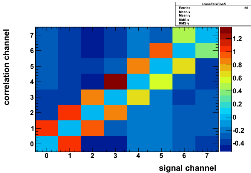
Figure 6. Cross-talk coefficient map of pads in area 1.
