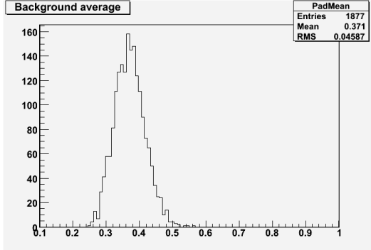
Figure 2. Background depositions in one pad of the Beamcal from about 2000 bunch crossings.
