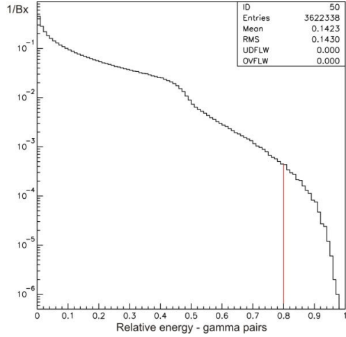
Figure 10. Distribution of energy of beamstrahlung pairs normalized to the nominal cms energy.
