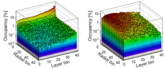
Figure 5. Left: the occupancy of energy deposition in LumiCal pads from incoherent pairs, with 0.2 MIP cut. Right: same for \gamma\gamma
