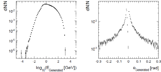
Figure 2. Distributions of energy (left) and of polar angle (right) of particles originating from \gamma\gamma background.
