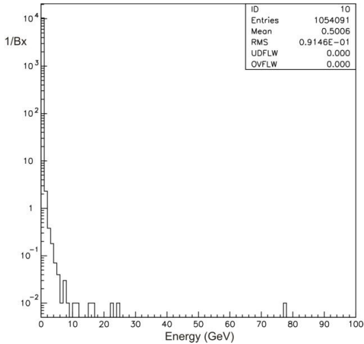
Figure 7. Energy distribution of incoherent pairs that enter the fiducial volume of LumiCal
