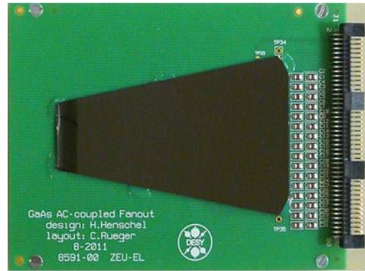
Figure 7. Sensor mounted on fan-out and instrumented by capacitances, resistors and connector.
