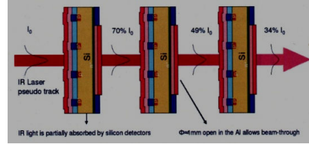
Figure 4. Schematic view of infra-red laser beam traversing several transparent sensors.
