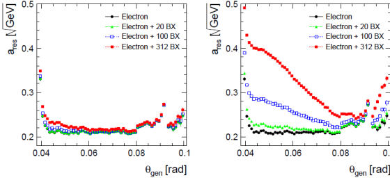
Figure 6. Measure of the energy resolution, a_{res} , as a function of the e^- polar angle, \theta_{gen} , without and with background, integrated over different number of BXs, as depicted in the figure. The left (right) plot presents results of incoherent pairs ( \gamma\gamma ) background.
