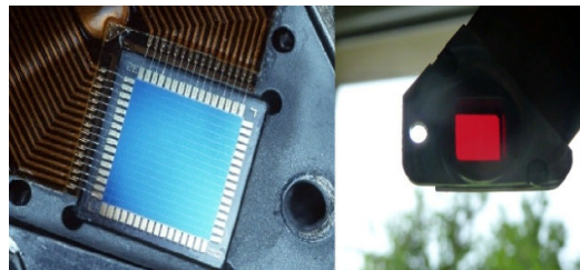
Figure 6. DPSD-516: Left: Sensor bonding to flat, readout cables: Right: A transparency to infra-red laser light.
