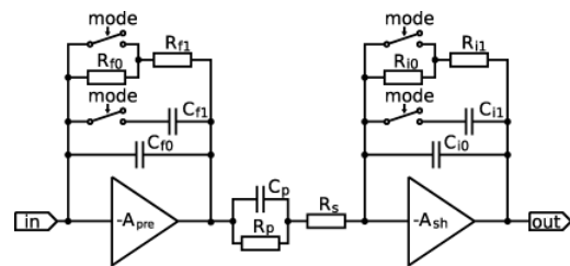
Figure 2. Block diagram of a single front-end channel.
