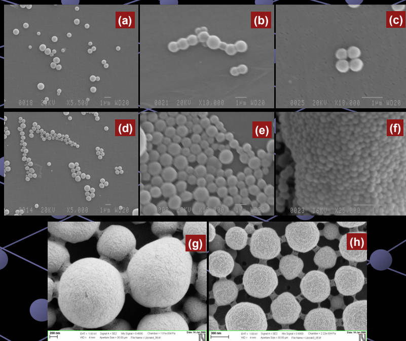
Figure 1: PLGA/HAp sphere-like particles: (a) individual, (b) linear, (c) tetragonal (d) pentagonal and part of the planar spatial arrangement of spheres. Morphology of composite spheres stabilized by PVP with (e) higher (650 kDa) and (f) lower (25 kDa) average molecular mass. Physical connections between sphere-like particles in PLGA/HAp composite with polymeric-to-ceramic part 75:25 (g) and 90:10 (h) stabilized by PVP with lower average molecular mass.
