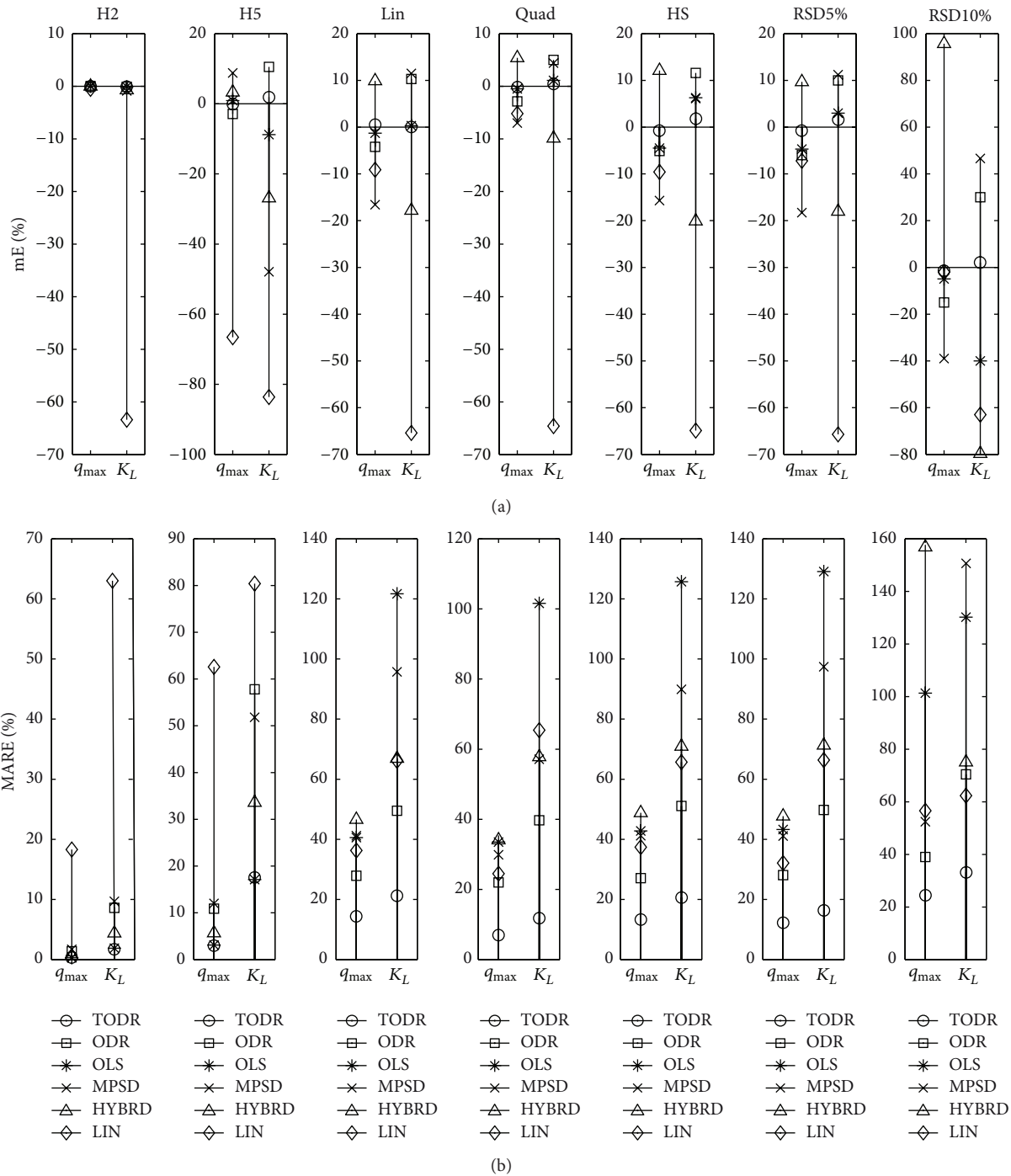
FIGURE 4: Properties of different modeling approaches for determination of parameters in Langmuir isotherm (experiments performed once): (a) mE and (b) MARE.
