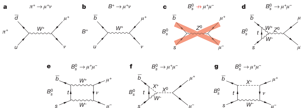
Figure 1 | Feynman diagrams related to the B_s^0 \rightarrow \mu^+ \mu^- decay. a , \pi^+ meson decay through the charged-current process; b , B^+ meson decay through the charged-current process; c , a B_s^0 decay through the direct flavour changing neutral current process, which is forbidden in the SM, as indicated by a large red
