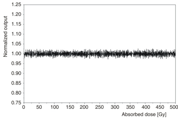
Figure 5. Normalized LED stability vs. absorbed dose
