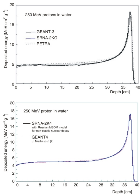
Figure 5. Monte Carlo simulation of depth-dose distribution in water for 250 MeV proton beams
