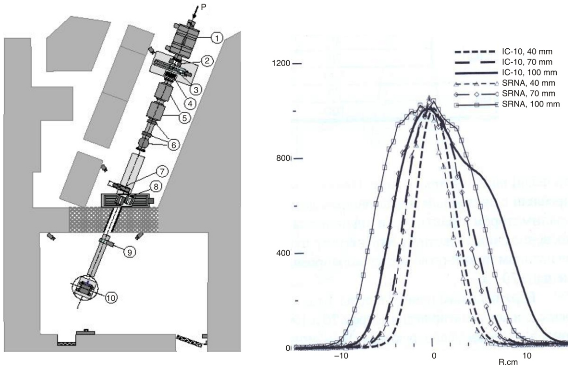
Figure 11. Cross-section of the INR (Troitzk, Russia) proton beam
