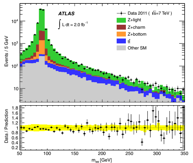
FIG. 1 (color online). e^+e^- invariant mass distribution for events passing the Z + \geq 1 jet selection, before imposing the |m_{ee} - m_Z| < 15 \text{ GeV} requirement. The predicted contributions of the SM background sources are shown stacked. The lower panel shows the ratio of the data to the SM prediction, and the solid band denotes the systematic uncertainty on the SM prediction.
