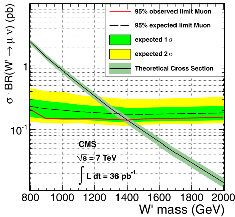
Fig. 4. The expected and observed 95% C.L. limits for the W' \rightarrow \mu\nu channel with the one and two sigma uncertainty band for the expected limit including the systematic uncertainties. Also shown is the NNLO cross section for the considered model including PDF uncertainties.
