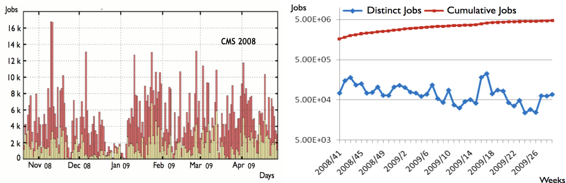
Figure 11. CRAFT jobs distributions as a function of time. Left: Daily distribution of analysis jobs submitted using CRAB and accessing CRAFT data. Grid (dark shading, red) and CAF (light shading, yellow) activities are shown. (Taken from monitoring sources). Right: CRAFT jobs submitted only at CAF (with and without CRAB). The upper line shows the cumulative number of jobs, the lower line shows the number of jobs submitted each week. The time window extends well beyond the end of CRAFT data taking to cover the extensive period of analysis.
