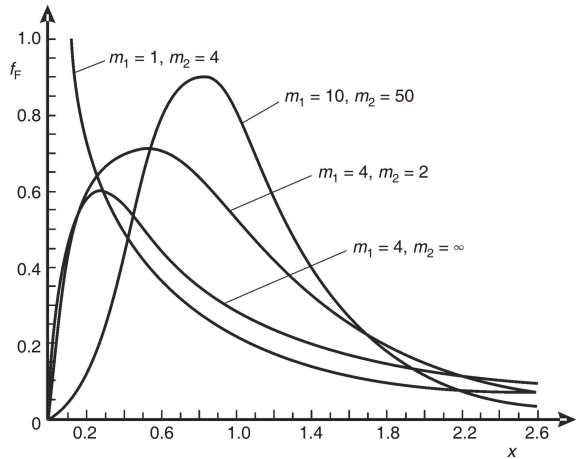
Figure 1. Probability density function characteristic f_F(x) of F distribution with m_1 and m_2 degrees of freedom as parameters
