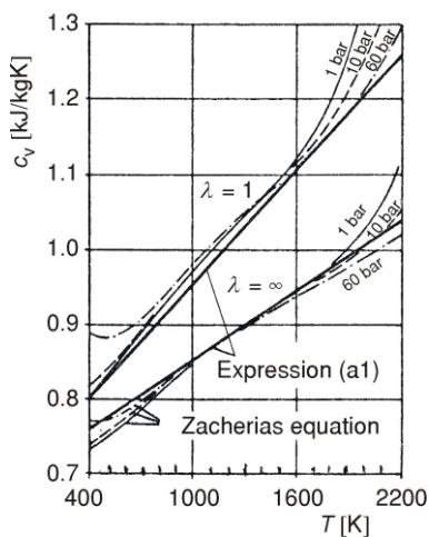
Figure A1. Comparison of specific heat according to Zacharias and expression (a1) [9]
