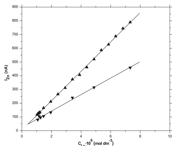
Figure 4. Dependence of Zn (II) peak current on added Lu (III) in the range [Lu] = (1 - 7.3) \cdot 10^{-6} M, and deposition time: (▼) 10 s; (▲) 30 s. The initial [Zn-EDTA] was 3.6 \cdot 10^{-5} M. Supporting electrolyte: 0.2 M NaClO 4 in 0.05 M pH 5.4 sodium acetate buffer; deposition potential: -1.200 V; sweep rate: 10 mV s -1 .
