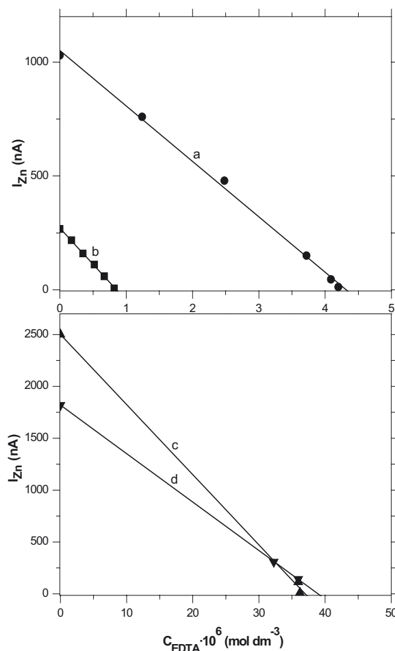
Figure 2. Dependence of Zn (II) peak current on added EDTA for different initial [\text{Zn}] and deposition times ( t_{\text{dep}} ): (●) [\text{Zn}] = 4.2 \cdot 10^{-6} M, t_{\text{dep}} = 90 s; (■) [\text{Zn}] = 8.2 \cdot 10^{-7} M, t_{\text{dep}} = 120 s; (▲) [\text{Zn}] = 3.6 \cdot 10^{-5} M, t_{\text{dep}} = 30 s; (▼) [\text{Zn}] = 3.6 \cdot 10^{-5} M, t_{\text{dep}} = 10 s. Supporting electrolyte: 0.2 M \text{NaClO}_4 in 0.05 M pH 5.4 sodium acetate buffer; deposition potential: -1.200 V; sweep rate: 10 \text{ mV s}^{-1} .
