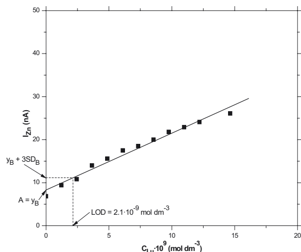
Figure 5. Graphical representation of limit of detection (LOD) determination: (A) – intercept of the calibration line; y_B – calculated blank; SD_B – estimated blank standard deviation; [Lu] = (1 - 15) \cdot 10^{-9} M. Initial [Zn-EDTA] was 8.2 \cdot 10^{-7} M. Supporting electrolyte: 0.2 M NaClO_4 in 0.05 M pH 5.4 sodium acetate buffer; deposition potential: -1.200 V; deposition time: 120 s; sweep rate: 10 mV s^{-1} .
