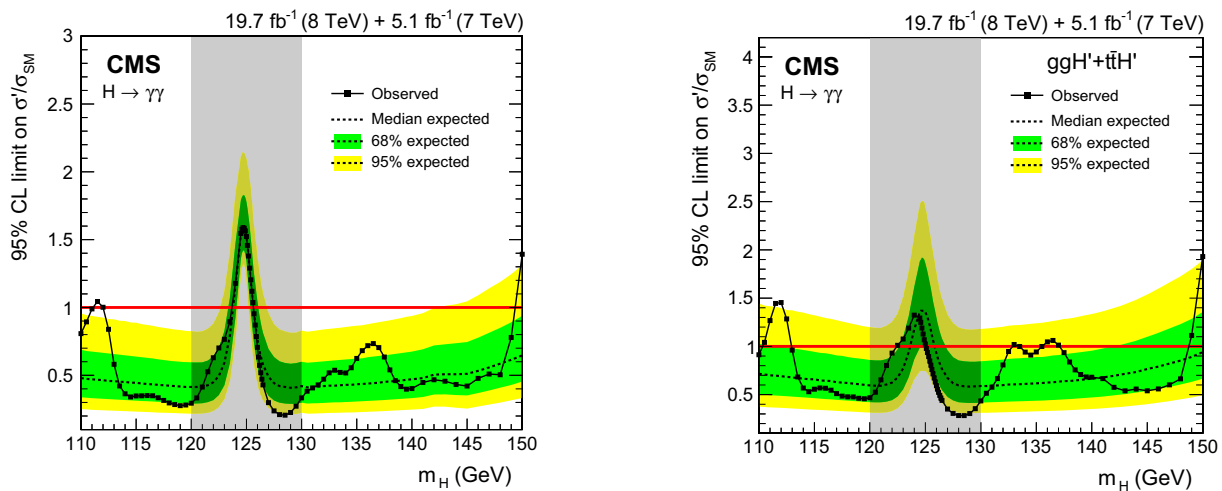
Fig. 27 Exclusion limit on the signal strength, \sigma'/\sigma_{SM} , for a second Higgs-boson-like state with SM couplings taking the observed state at 125 GeV as part of the background. The shading indicates a window with a width of 10 GeV, centred at the best-fit mass, where the expected sensitivity to a second Higgs boson is severely degraded due to the presence of the already observed state
