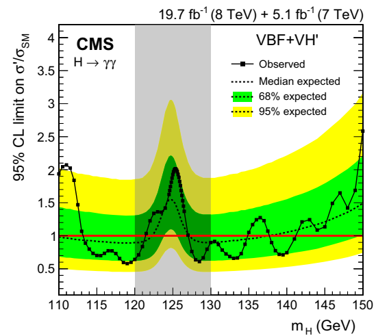
Fig. 28 Exclusion limits on \sigma'/\sigma_{SM} for a second Higgs-boson-like state produced with gluon–gluon fusion only (top) or VBF and VH only (bottom) taking the observed state at 125 GeV as part of the background. The shading indicates a window with a width of 10 GeV, centred at the best-fit mass, where the expected sensitivity to a second Higgs boson is severely degraded due to the presence of the already observed state
