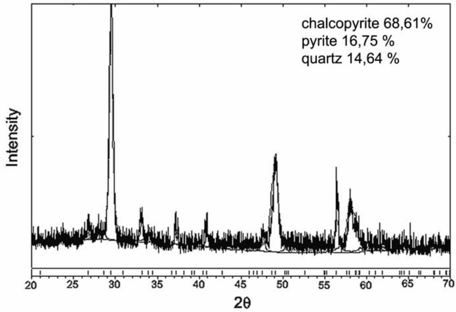
Figure 1. Diffractogram of Charge 3 sample
