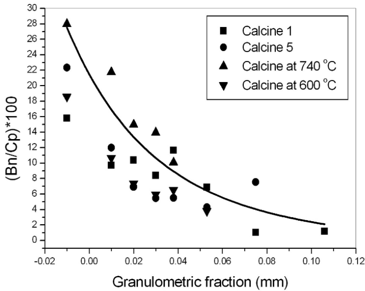
Figure 7. Effect of grain size on transformation degree (Cp - chalcopyrite ( \text{Cu FeS}_2 ), Bn - bornite ( \text{Cu}_5\text{FeS}_4 ))
