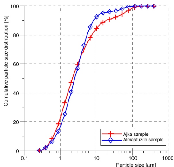
Figure 2. Particle size distribution of red mud samples
