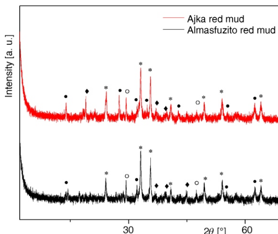
Figure 1. XRD patterns of the red mud samples; hematite ( \text{Fe}_2\text{O}_3 ) – marked by a solid star symbol, calcite ( \text{CaCO}_3 ) – marked by a clear circle symbol, cancrinite ( \text{Na}_6\text{Ca}_2\text{Al}_6\text{Si}_6\text{O}_{24}(\text{CO}_3)_2 ) – marked by a solid circle symbol, gibbsite ( \text{Al}(\text{OH})_3 ) – marked by a solid rhombus symbol)
