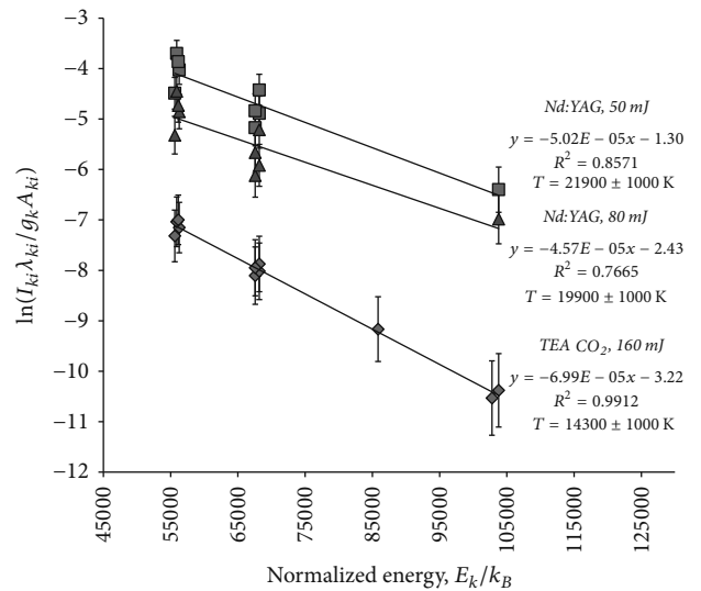
FIGURE 4: Boltzmann's plot for laser-induced plasma of basalt at atmospheric pressure utilizing Fe II transition lines listed in Table 1. T_{\text{exc}} = -1/\text{Slope} . The error bars account for combined uncertainties of line intensity measurements and of transition probability accuracy (Table 2).
