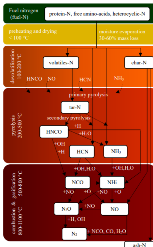
Fig. 1. Conversion of fuel-N (biomass combustion)
