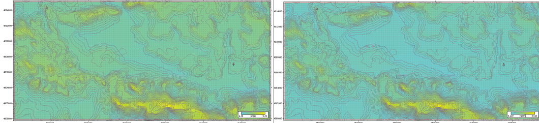
Figure 8. Guševac 30 m – Wind speed (2.40-8.39 m/s) and AEP (0.230-8.555 GWh) fields
