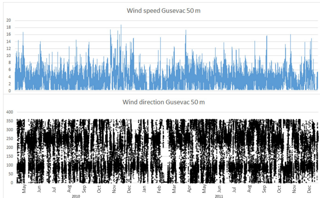
Figure 11. Observed wind speed and direction for the site Guševac 50 m
