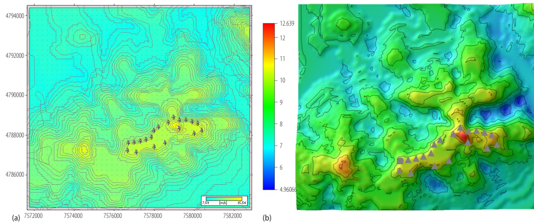
Figure 2. Mean wind speed fields obtained by simulations in WAsP (a) and WindSim (b) (for color image see journal web site)
