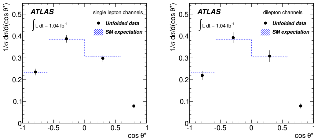
Figure 5. Unfolded distributions of \cos\theta^* for the (left) single-lepton and (right) dilepton channels. The error bars on unfolded data (markers) include both the statistical and systematic contributions. For comparison, the Standard Model NNLO QCD prediction (dashed line) and its uncertainty [4] are also shown.
