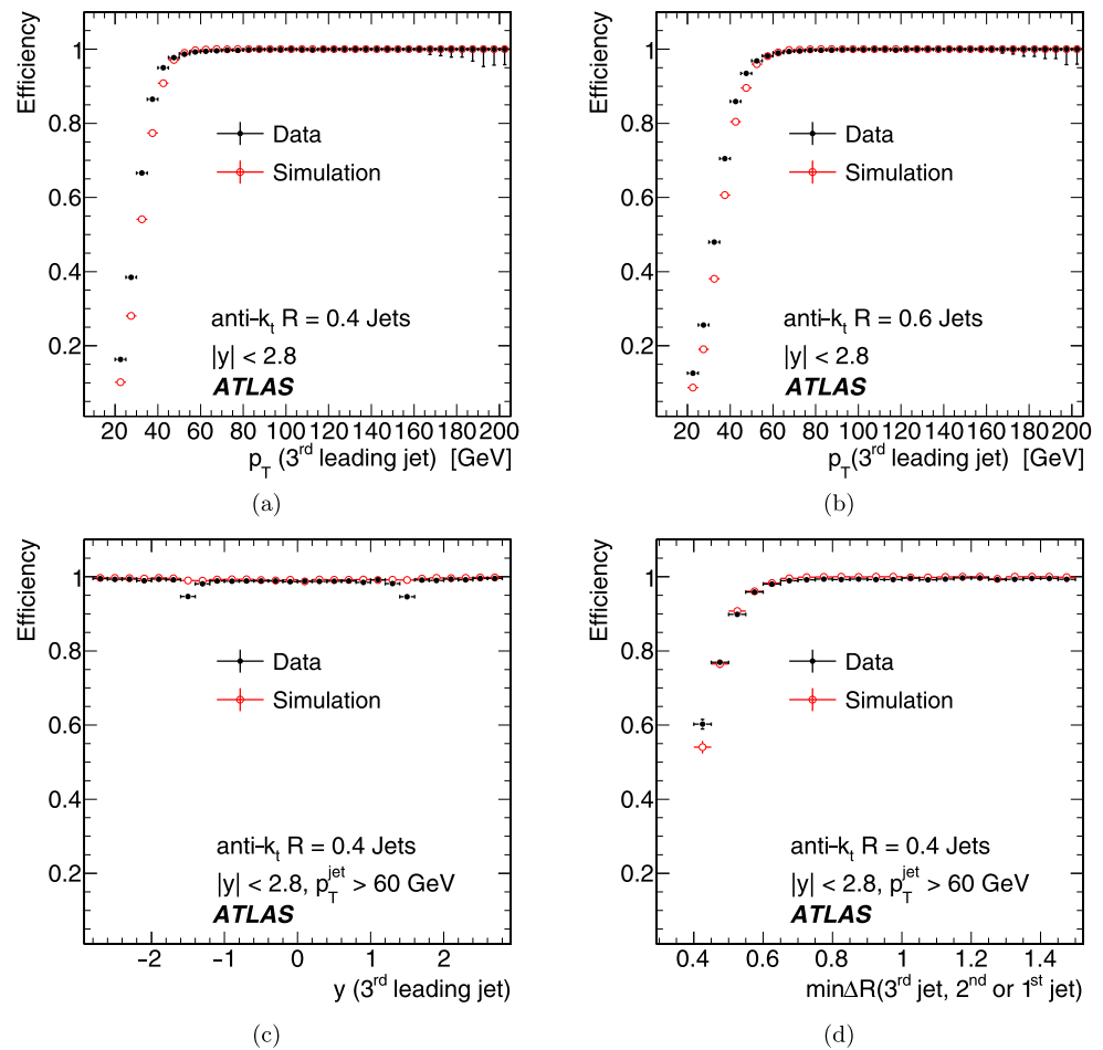
Fig. 1 Jet trigger efficiency for the third leading jet as a function of p_T for anti- k_t jets with R = 0.4 (a), and R = 0.6 (b). Jet trigger efficiency as a function of y of the third leading jet with p_T > 60 GeV and R = 0.4 (c). Jet trigger efficiency as a function of the minimum separation \Delta R between the two closest jets (d). The efficiency is shown both as calculated in data, as described in the text, and in Monte Carlo simulations for the three-jet trigger with a level-1 cut on the jet transverse energy of 10 GeV
