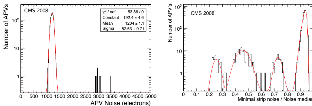
Figure 4. (Left) Mean calibrated noise for individual APV25 chips on modules in the TOB single side layer 3. (Right) The ratio of minimum noise to median noise per APV25 chip. The distinct populations reflect the different noise sources within a module.
