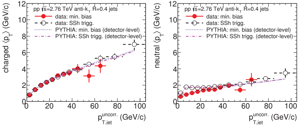
Fig. 76. Mean transverse momentum, \langle p_T \rangle , of constituents measured in reconstructed jets in 2.76 TeV pp collisions (anti-kT, R = 0.4 ) versus jet p_T . Left: charged tracks; Right: neutral clusters. Data are shown for MB and SSh triggers, and are compared to detector-level simulations.
