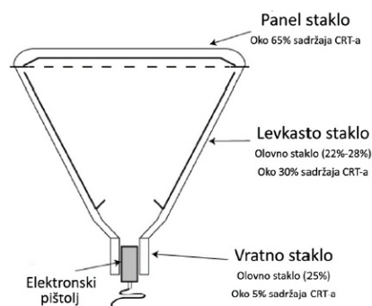
Figure 2. CRT scheme [12]
