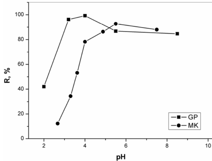
Fig. 7. Influence of pH value on removal efficiency of MK and GP (0.1 g MK/GP, 50 mg/dm 3 Pb, 60 minute).
