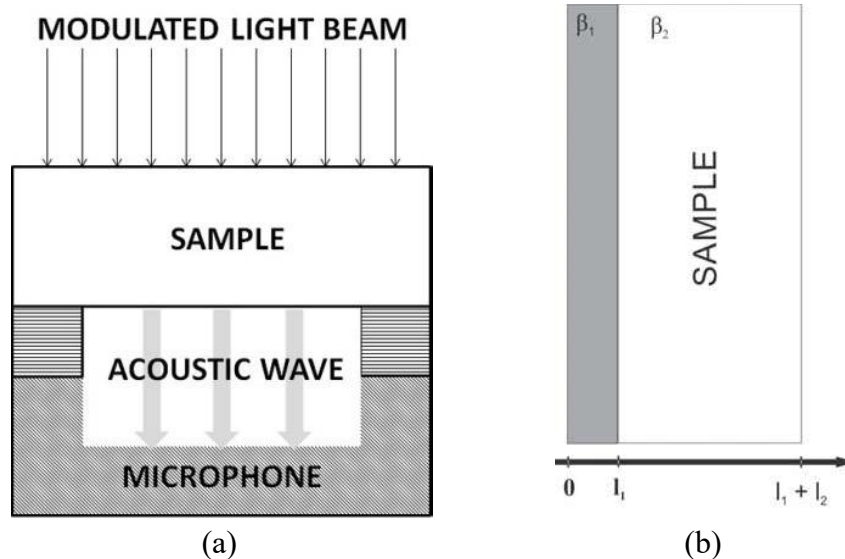
Figure 1. a) Transmission experimental configuration, b) Two-layered sample.
